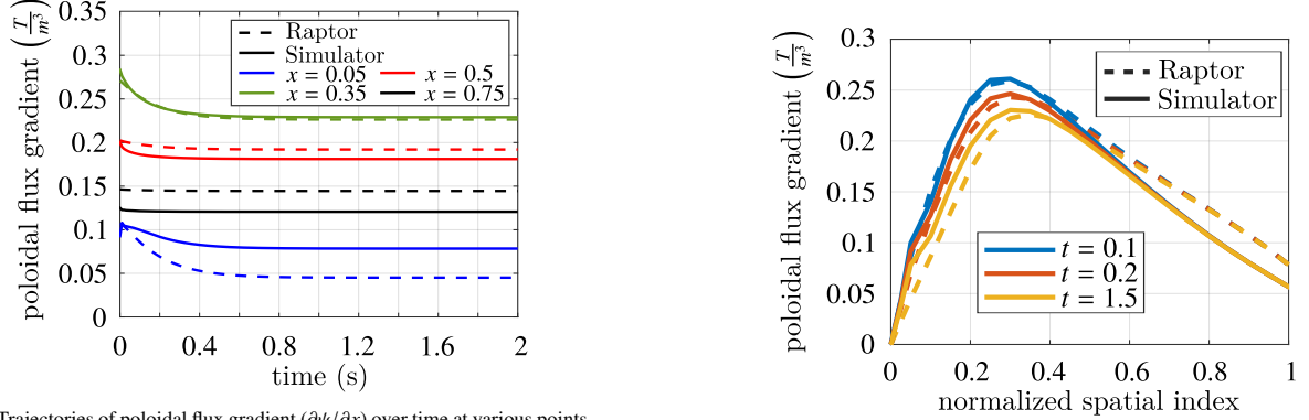
(a) Trajectories of poloidal flux gradient ( \partial\psi/\partial x ) over time at various points of the normalized spatial index \{0.05, 0.35, 0.5, 0.75\} . The dashed lines represent trajectories obtained from an open-loop Raptor simulation, while the solid lines depict trajectories resulting from the simulator proposed in this study.
