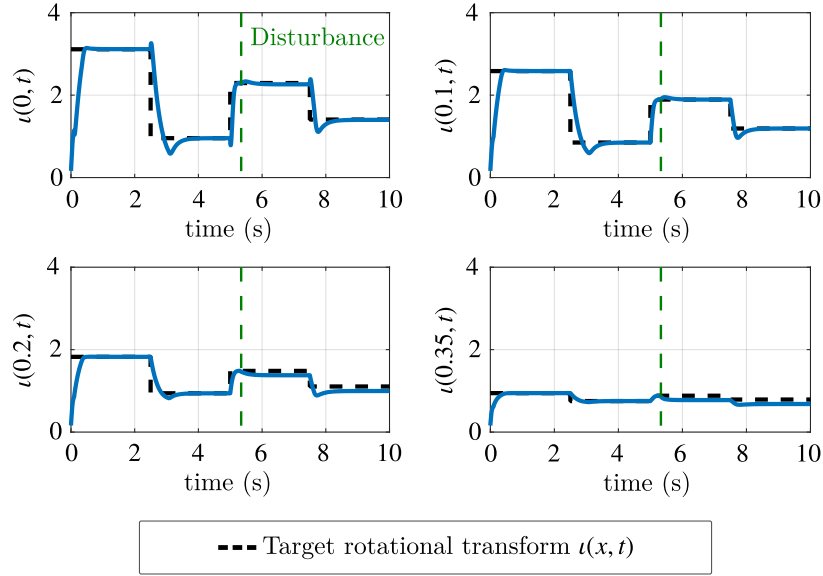
Fig. 11: Rotational transform profiles ( u(x, t) ) at different points of the spatial domain \{0, 0.1, 0.2, 0.35\} for a time period of 10 seconds. A disturbance, implemented as a Neutral-Beam Injector placed in a different place from the ECCD antenna control input, is applied at time t = 5.3 (s). In this simulation the position at which we want to regulate the error to zero is x = 0.1 , while the controller was trained to regulate the error at x = 0.2 .
