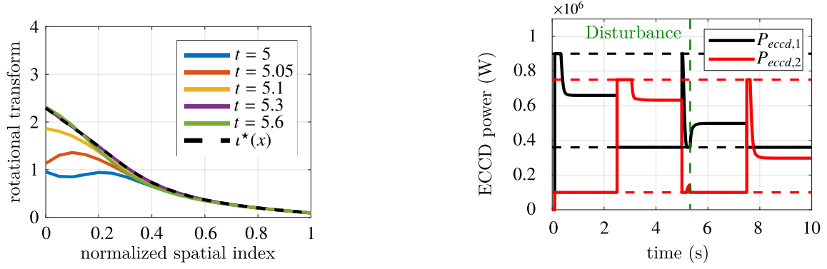
(a) Rotational transform profiles ( \iota(x, t) ) at different time instants after the disturbance application.
