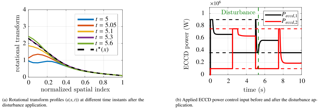
Fig. 10: l -profiles and applied ECCD power ( P_{ECCD,i} ) for the two antennas in case of external disturbance application.
