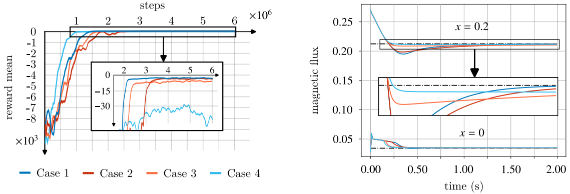
(a) Reward mean of four different training of the proposed RL algorithm.
