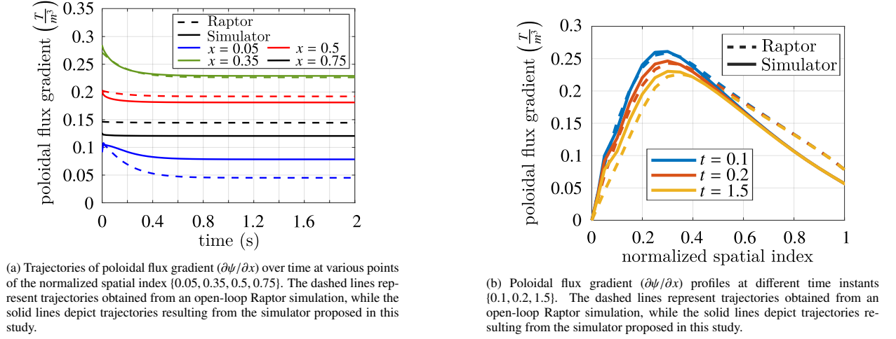
Fig. B.13: Comparison between Raptor and training model open-loop simulations.
