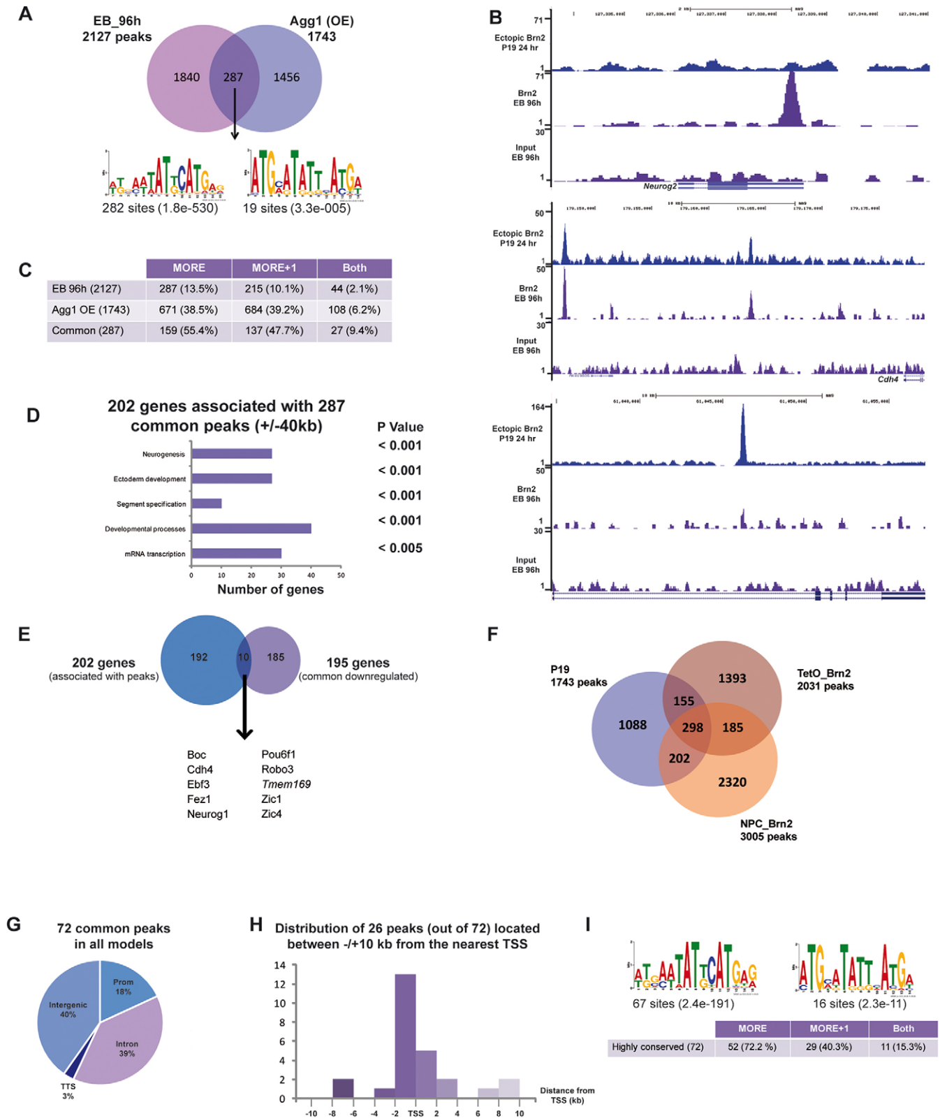
Fig. 5. Comparison of Brn2-occupied sites in retinoic-acid-treated embryoid bodies and P19 cells. (A) Venn diagrams indicating the overlap between the Brn2 sites in the indicated data sets. A MEME-ChIP analysis of the commonly occupied sites shows an enrichment in MORE-like motifs. (B) UCSC screenshot showing representative examples of common and specific peaks. (C) Table indicating the frequency of the indicated motifs at common and specific sites. (D) Ontology of the genes associated with the Brn2 sites commonly occupied in embryoid bodies and P19 cells. (E) Venn diagram indicating the overlap between genes associated with Brn2-occupied sites and downregulation following shBrn2 silencing in embryoid bodies and P19 cells. (F) Venn diagram indicating the overlap between genes associated with Brn2-occupied sites in P19 cells and NPCs with or without ectopic Brn2 expression. (G) Pie-chart showing distribution of the core set of 72 Brn2 sites in the genome. (H) A subset of core sites are enriched around the TSS. The graph shows a plot of the frequency of Brn2-occupied sites versus the distance to the TSS. (I) Core sites are highly enriched in MORE-like motifs.
