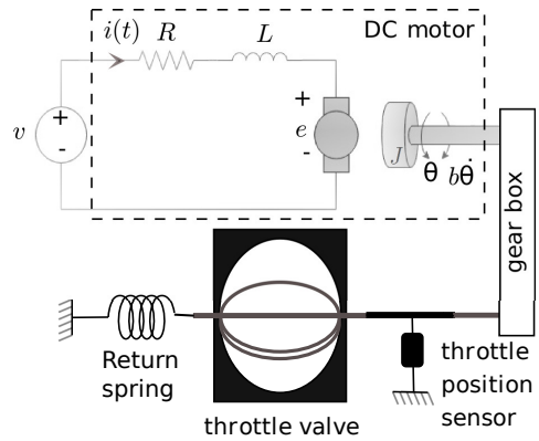
Figure 2: Block diagram of the valve.
