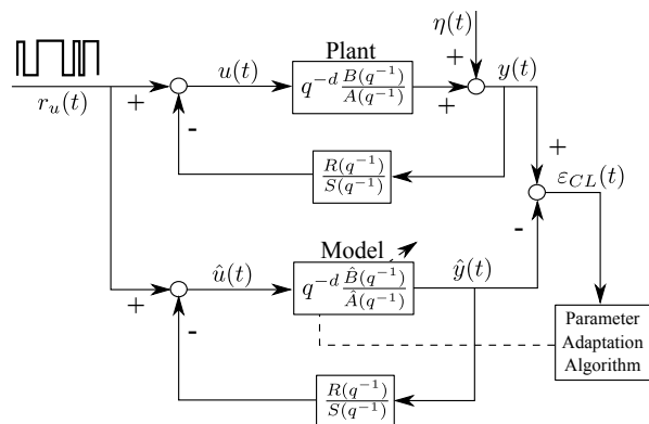
Figure 11: Identification in closed loop. Excitation is superposed to control output.
