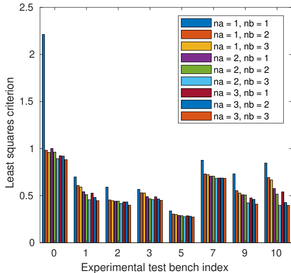
Figure 5: Normalized least-squares criterion (7) for different combinations of the number of free parameters of the model (varying both the number of past outputs n_a and past inputs n_b used for the predicted output). The same computations are carried out for each valve and presented in parallel. While increasing the number of parameters improves the accuracy, the model obtained with n_a = n_b = 1 gives reasonable results for most of the valves.
