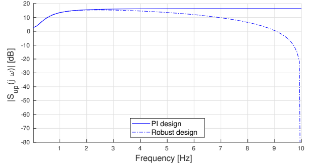
Figure 8: Input sensitivity function for the robustness analysis ( a_1 = 0.9152; b_1 = -0.0609 ). Plain lines: PI design setting the closed-loop behavior as a damped 2^{nd} order dynamics; dashed lines: robust design when opening the loop at 0.5 f_s . High-frequency disturbances are removed from the control signal by the robust design.
