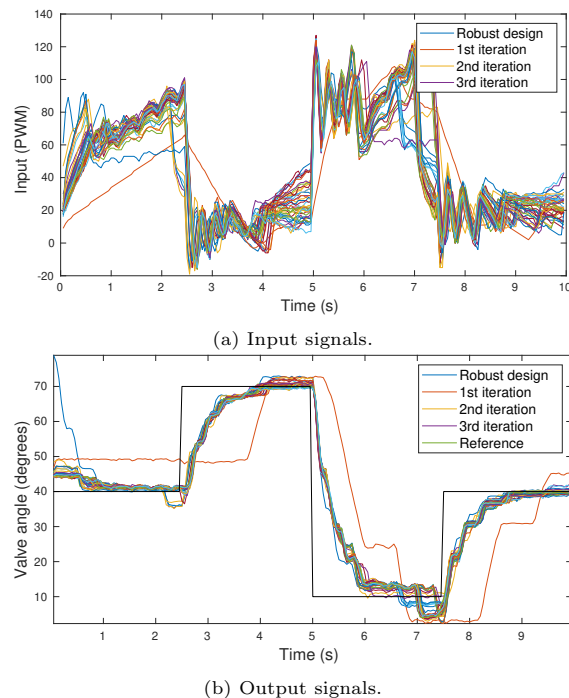
Figure 12: Performance evaluation of the adaptive method iterative identification in closed loop and controller re-design on Experiment 6 . The response corresponding to the Robust control design is compared with successive iterations of the adaptive design. More accurate tracking is obtained with the adaptive method after a few iterations.
