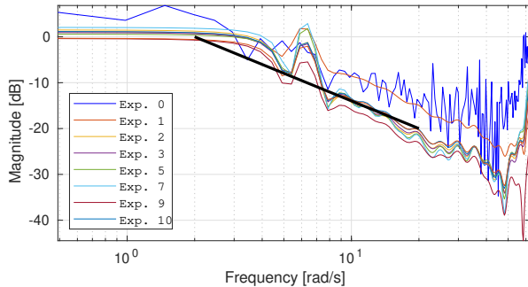
Figure 4: Empirical Transfer Function Estimate (ETFE) of the valves' responses to a PRBS input. The raw ETFE of Experiment 0 is depicted in dark blue while filtered values are shown in the other colors for all the valves. The black line follows a slope of -20dB/dec, which captures the main transient dynamics of the valves.
