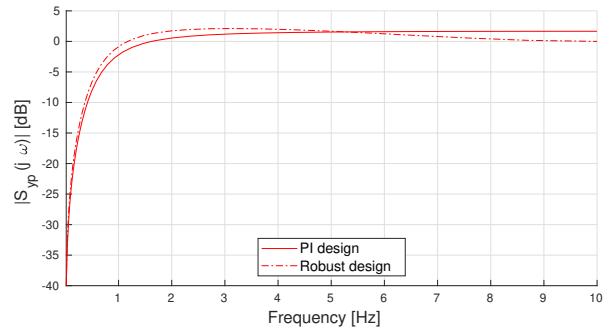
Figure 9: Output sensitivity function. The performance of the robust design is close to the one of the PI design.
