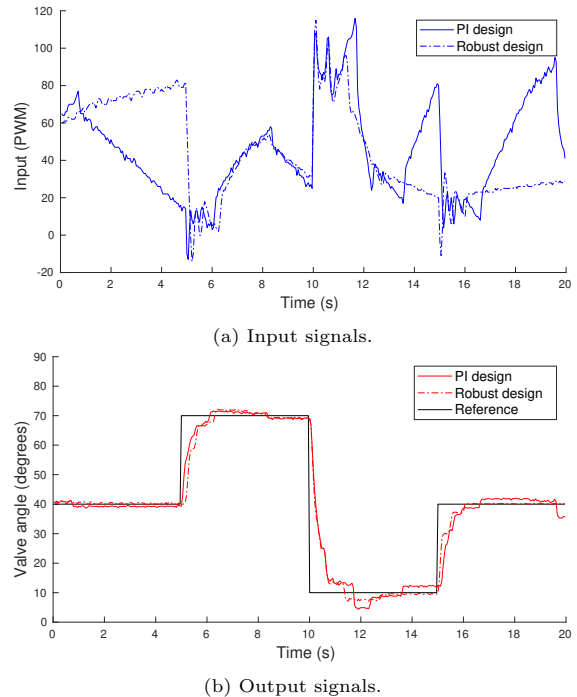
Figure 10: Evaluation of the robust design performance on Experiment 6 . Plain lines: PI design setting the closed-loop behavior as a damped 2 nd order dynamics; dashed lines: robust design when opening the loop at 0.5 f_s . Robustness does not impair the controller's performance.
