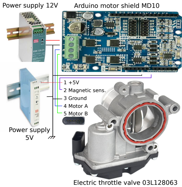
Figure 1: Experimental test bench of the throttle valve: power supply and wiring.
