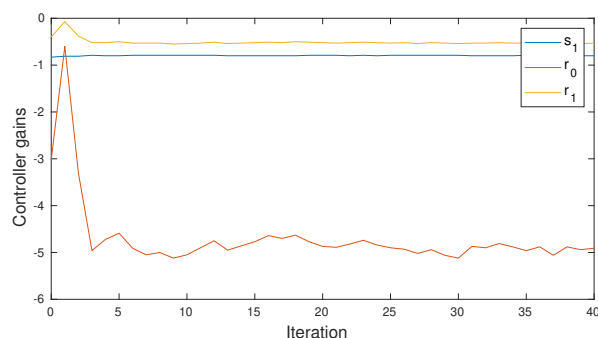
Figure 13: Evolution of the controller's gains during the iterations of the adaptive method.
