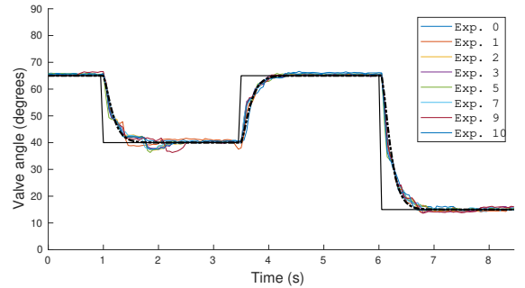
(b) Outputs for a target damping ratio of 1.0.
