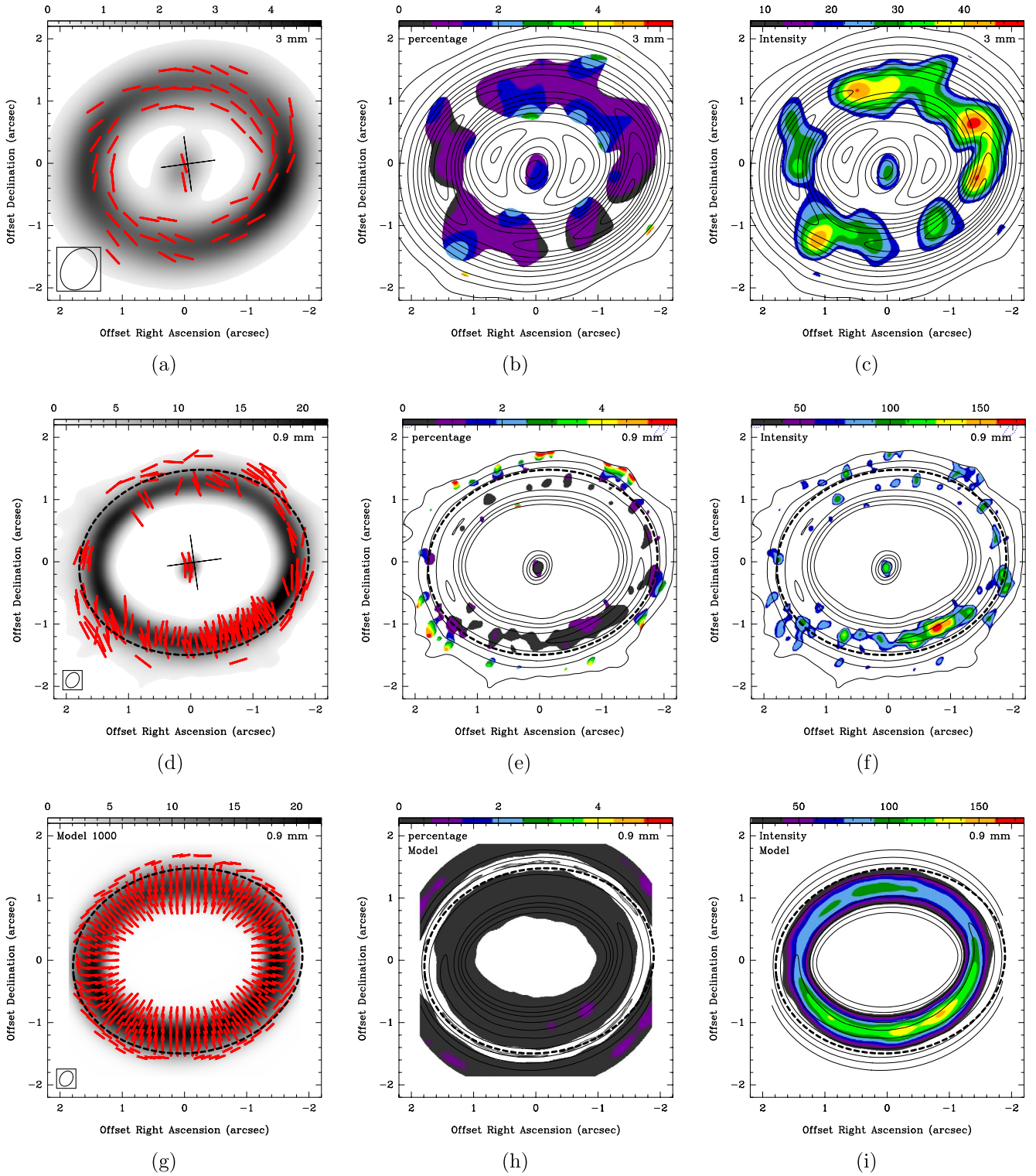
Figure 1. Panels (a), (d): detected polarization position angles shown in red segments and continuum emission in gray scale at 3 and 0.9 mm. Panels (b), (e): polarization percentages in color. Panels (c), (f): polarization intensity in color. The upper and middle panels are results from 3 and 0.9 mm, respectively. Panels (g)–(h) are the model images with a_{\max} of 1000 \mu\text{m} at 0.9 mm. The model polarization percentage is masked with a cutoff of 0.2%. Contours in panels (b), (c), (e), (f) denote -3, 3, 10, 20, 40, 60, \dots, 180, 200 \times \sigma_l . The wedge units are \text{mJy beam}^{-1} in panels (a), (d), (g), percentage in panels (b), (e), (h), and \mu\text{Jy beam}^{-1} in panels (c), (f), (i). The dashed ellipse in panels (d)–(i) marks the 1''.85 (280 au) radius. Polarization is only displayed for a signal-to-noise ratio in polarized intensity greater than 3.
