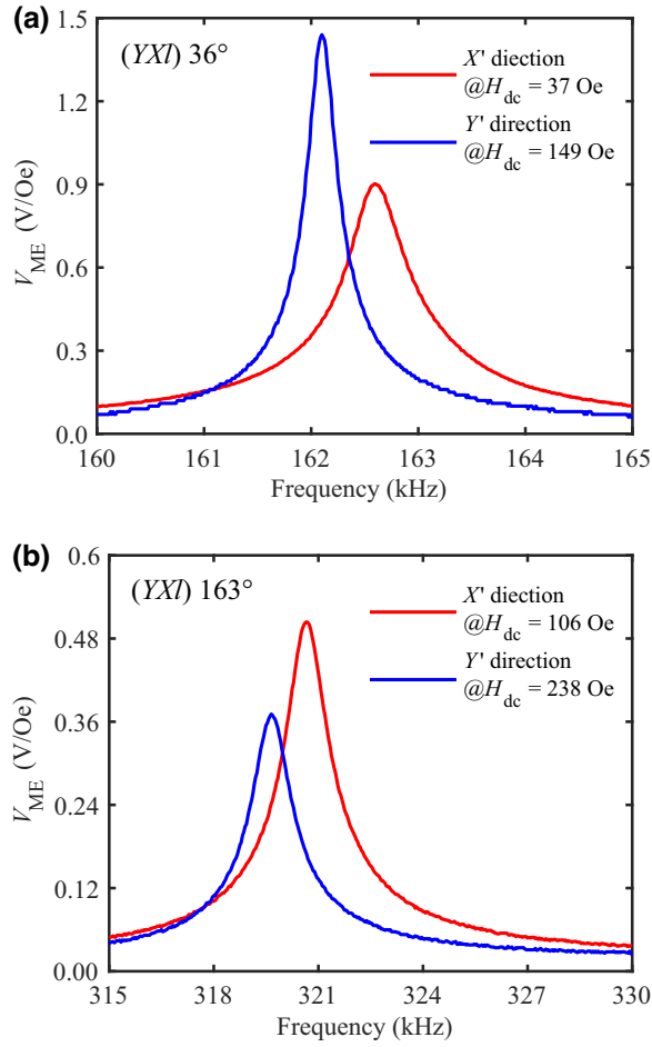
FIG. 4. ME resonance measurement as a function of frequency for (a) Ni/(YXl)36° LiNbO 3 /Ni and (b) Ni/(YXl)163° LiNbO 3 /Ni samples in X' and Y' directions.
