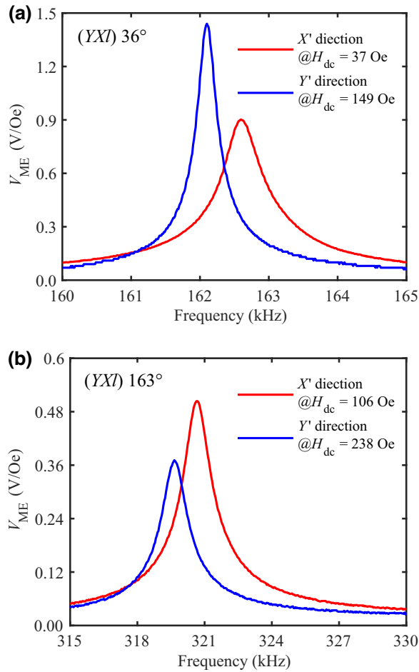
FIG. 4. ME resonance measurement as a function of frequency for (a) Ni/( YXl ) 36^\circ LiNbO 3 /Ni and (b) Ni/( YXl ) 163^\circ LiNbO 3 /Ni samples in X' and Y' directions.
