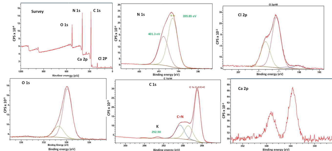
Figure 6. XPS analysis of CN.
