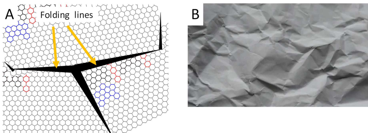
Figure 4: A) a simple model showing how foldings may give rise to different domains inside a single crystal flake. B) analogy with a folded sheet of paper.
