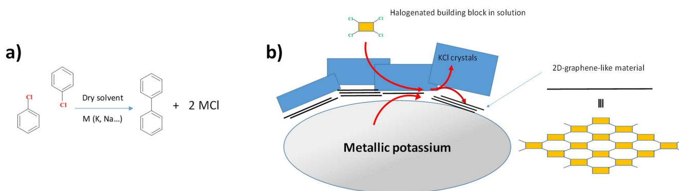
Figure 2: a) The Fittig reaction ; b) confining the growth of layered materials by both a surface and a metallic salt.
