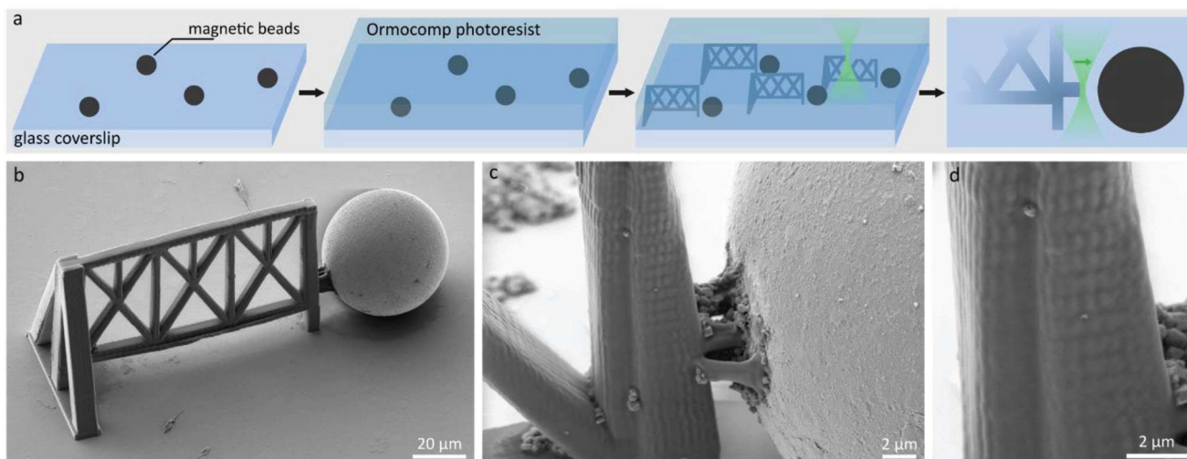
Figure 2. Printing of the OrmoComp skeleton bound to a NdFeB magnetic bead. a) Schematics showing the printing process: the beads are first dispersed on the coverslip and a drop of resin is deposited on top. The structures are then built next to magnetic beads, and linked to them. b) scanning electron microscope (SEM) image of a magnetic bead attached to the OrmoComp skeleton. c) Zoom on the OrmoComp-made link. d) Details of the voxels on the structure.
