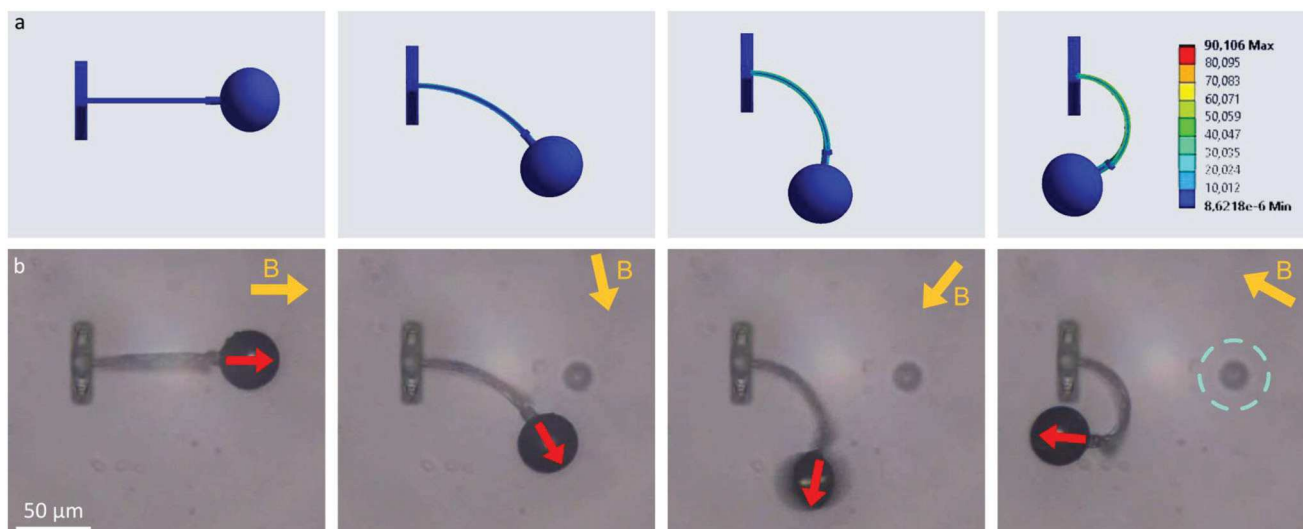
Figure 3. Magnetic actuation of the skeleton. a) Non-linear finite elements simulation of the beam deflection and associated Von-Mises stress (values expressed in MPa in the color scale). b) Optical microscope images of the skeleton deformation under a magnetic field (yellow arrow: external magnetic field; red arrow: bead magnetization; circled area: printing artifact, which may block the movement).
