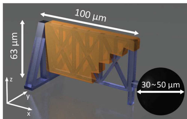
Figure 1. 3D rendering of the global structure. Blue: internal OrmoComp skeleton; orange: hydrogel envelope (cutout to reveal the skeleton); black: magnetic bead for actuation.
