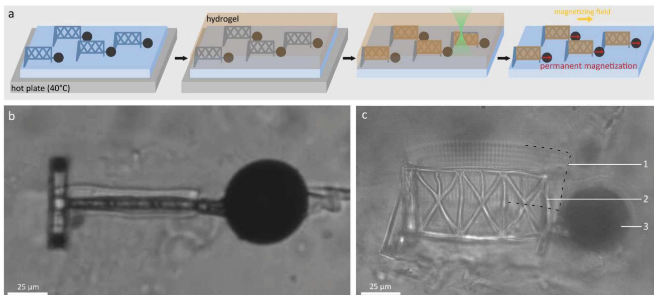
Figure 4. Printing the collagen envelope. a) Schematics showing the printing process: the sample is heated to 40 °C and a drop of liquid hydrogel is deposited on top of the structures. The system is kept at 40 °C for 30 min, then cooled back to room temperature. The envelopes are then printed around the skeletons, and washed in PBS. Lastly, the beads are magnetized. b) Optical microscope top-down view of a printed full structure (skeleton, envelope, magnetic bead). c) Side view of a purposefully knocked down structure. 1: hydrogel envelope, 2: OrmoComp skeleton, 3: NdFeB bead.
