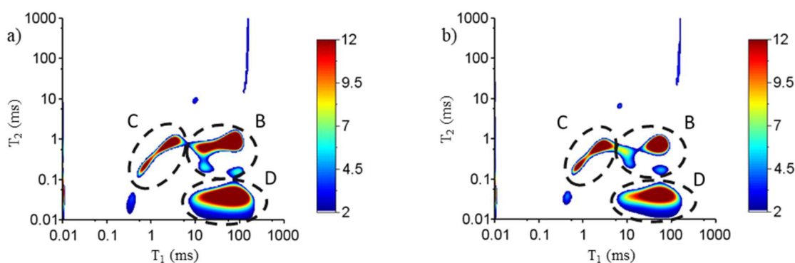
255 Figure 1. T_1 - T_2 correlation spectra of modern oak wood (a) and historical oak wood (b) samples by 2D ^1\text{H} T_1 - T_2 256 NMR relaxometry at 65% RH. Peaks B and C are attributed to ^1\text{H} detected from bound water and peak D is 257 attributed to ^1\text{H} from wood polymers. It should be noted that to follow previous notation (Cox et al. 2010) peak 258 A is not included here, which correspond to free water and it is not present in these samples. All the T_1 - T_2 259 correlation spectra acquired in this work can be found in Figures S3 and S4.
