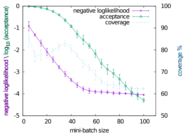
Figure 3: PBNN performance measured by \overline{\text{NLL}}_{\mathcal{D}} over the test data set, acceptance in base \log_{10} and one sigma coverage in function of the mini-batch size N for a constant prior. The standard deviation continuously decreases in function of the batch size. We notice however that the coverage is not monotonous: it is determined by both the error bars size and by the loglikelihood.
