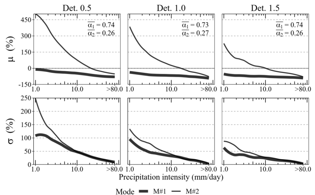
Figure 10. Sensitivity of GMM (with M = 2 ) mean ( \mu , upper panels) and standard deviation ( \sigma , bottom panels) parameters as a function of the precipitation ( x -axis, in \text{mm day}^{-1} ) and according to different PMW detection thresholds of 0.5, 1.0, 1.5 \text{mm h}^{-1} (from left to right panels), from the GIRAFE precipitation product. The weight ( \alpha ) parameters, for both the M#1 and M#2, are shown in the top right of the figure (upper panels) and represent their respective averages as a function of precipitation.
