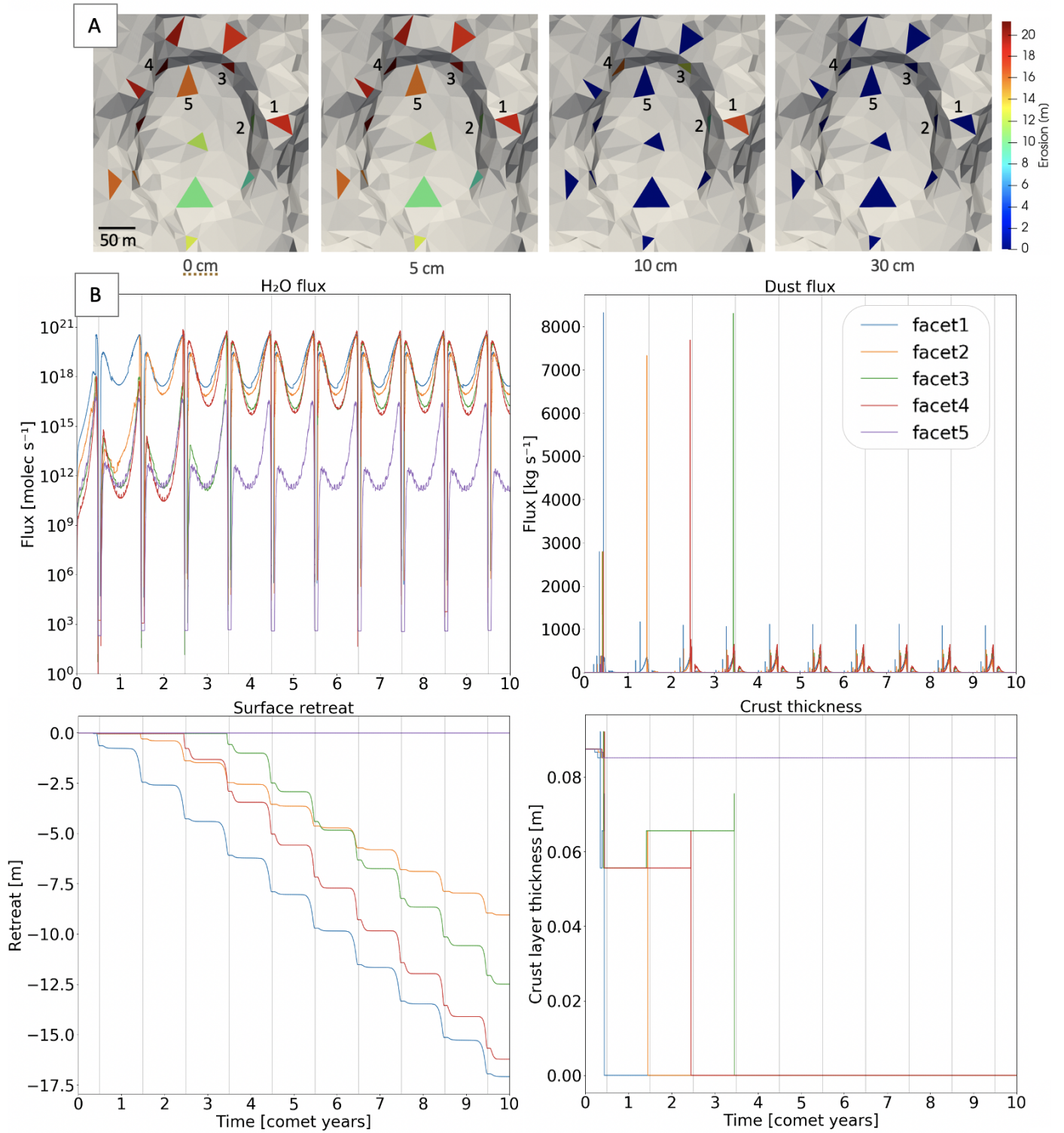
Fig. 10. Influence of the presence of a dust mantle. A: the erosion sustained after ten revolutions with an initial dust mantle of 0, 5, 10 and 30 cm, left to right , respectively. B: the H 2 O production rate, the dust production, the progressive erosion, and the thickness of the dust layer, given for five facets, for an initial dust mantle of 10 cm.
