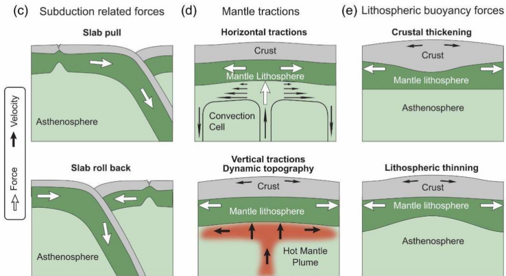
Fig. 1 | Driving forces, resisting factors, and weakening processes that accompany rifting. (a) Continental rifts are affected by a multitude of processes ranging from plate-tectonic driving forces to crustal faulting and surface processes. (b) Strength profile of the crust and lithosphere, showing the relatively lower yield strength imposed by the presence of mechanical anisotropy. (c-e) Simplified representation of major forces that drive continental rifting.
