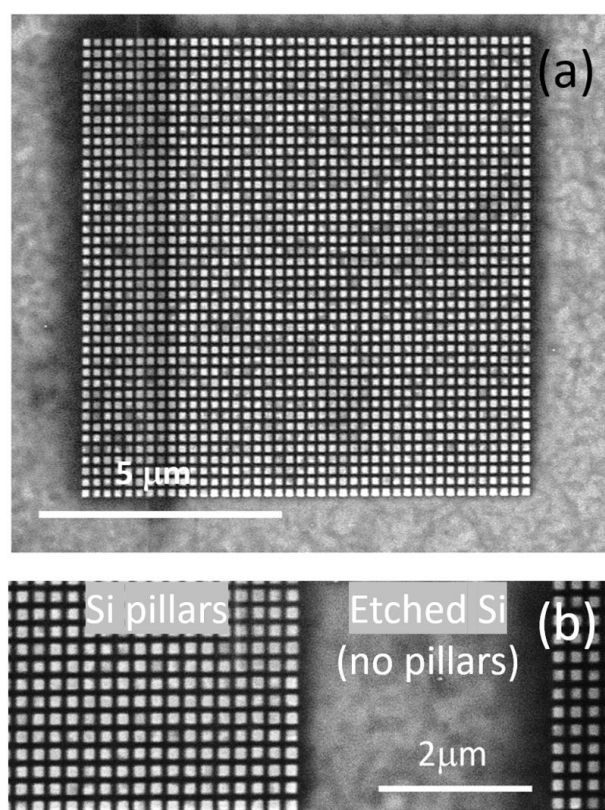
Fig. 2. (a) Scanning electron microscopy image of a complete Mie resonator etched onto silicon, on a silicon-on-sapphire substrate, and covered by the perovskite QDs layer. (b) Scanning electron microscopy image at the border between two Mie resonators with different ( L, g ) parameters highlighting the quality of the pillars and the presence of a flat silicon surface (i.e. with no pillars) in between.
