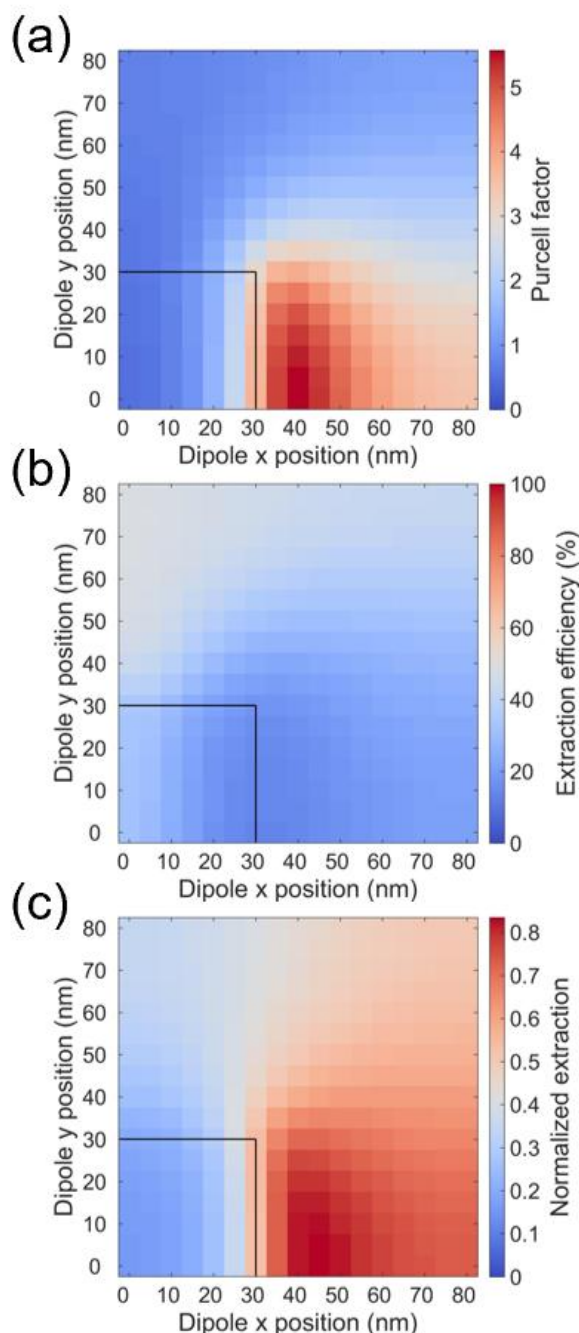
Fig. 3. (a) Simulated Purcell factor as a function of dipole position. (b) Simulated extraction efficiency as a function of dipole position. (c) Simulated overall extracted intensity, normalized by dipole emission, as a function of dipole position within the Mie resonator. Note that this magnitude combines the effect of Purcell enhancement (or inhibition) and extraction due to the Mie resonator. The dipole is x -polarized and radiates at 532 nm. The (L, g) parameters for this structure are (60, 100) .
