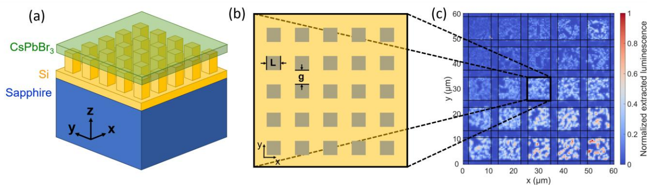
Fig. 1. (a) Schematic representation of the CsPbBr 3 layer deposited on Mie resonators, each corresponding to a set of (L, g) parameters. (b) Geometric parameters defining the size of the square pillars ( L ) and their side-to-side separation, which we refer to as the gap ( g ). (c) Perovskite luminescence, normalized to the maximum intensity of the image, over Mie resonators with varying (L, g) parameters.
