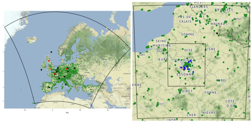
Figure 1. The simulations are run on a triple-nested configuration with a European domain with a 30 km resolution (FAIR30), an intermediary domain with a 10 km resolution (PAR10) and the finest domain focused on the Parisian region with roughly 3 km resolution (PAR03). Green circles are the EEA stations, red diamonds represent EBAS stations for \text{NH}_4^+/\text{NO}_3^- measurements, black downward triangles show WOUDC OzoneSonde stations and blue triangles show météo-France stations used in this study. Ozone Sonde stations are not located in the two inner domains. Data were extracted from the E-OBS gridded fields by using the locations of EEA stations; therefore, stations for both are similar (green points).
