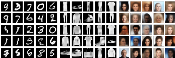
Figure 5: Generated sample obtained through a pre-trained decoder + RealNVP.
