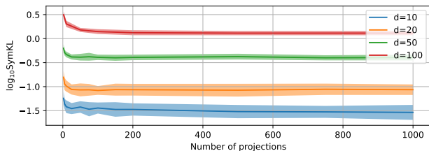
Figure 3: Impact of the number of projections for a fixed number of epochs.
