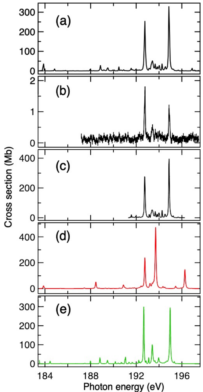
FIG. 4. Photoionization cross-sections of S^{4+} in 2p^63s3p^3P_{0,1,2} initial states: (a) measured, (b) and (c) simulated from the results of MCDF and R-Matrix theoretical calculations, respectively.
