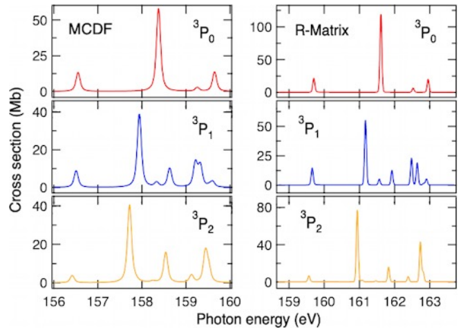
FIG. 3. Ab initio MCDF and R-Matrix cross sections for the h\nu + 2s^2 2p^6 3s 3p \ ^3P \rightarrow 2s^2 2p^5 3s^2 3p \ ^3L^e resonances after convolution with a Gaussian function of FWHM 64 meV to simulate the effect of instrumental broadening.
