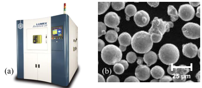
Fig. 1 (a) Matsuura Lumex Avance-25 (4 th generation) hybrid powder bed fusion system and (b) Matsuura maraging steel powder.
