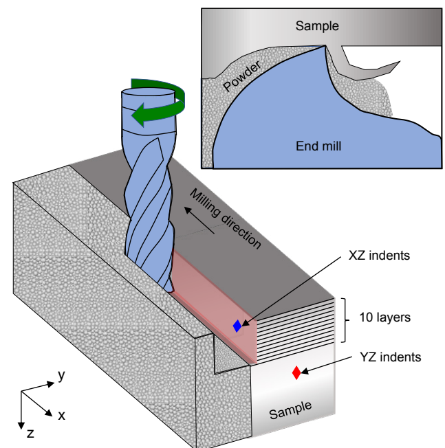
Fig. 2 Milling in powder.
