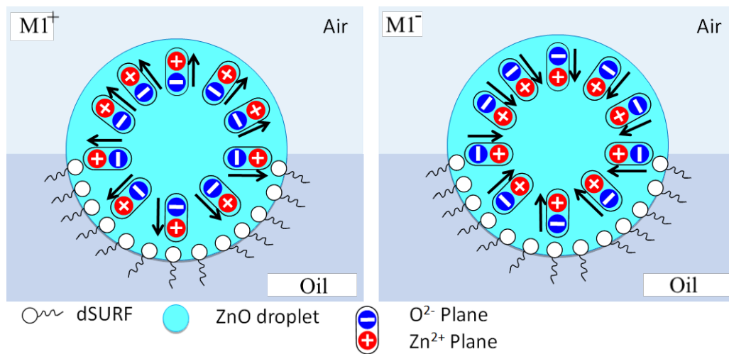
Figure 8. Schematic illustration of ZnO NP organizations leading to positively charged droplets (MI + , left) and negatively charged droplets (MI - , right) charged droplets, respectively. The coexistence of both organizations is mandatory to explain the observed square lattice of droplets.
