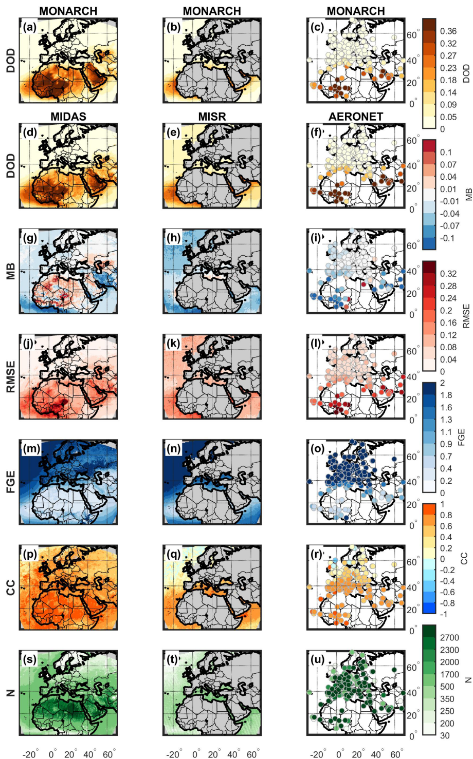
Figure 4. Spatial distribution of the total DOD simulated by the MONARCH reanalysis (a–c) and collocated with observations by MIDAS (d), MISR (e), and AERONET (f), along with the respective statistic parameters, including MB (g–i), RMSE (j–l), FGE (m–o), and CC (p–r). The number N gives the total number of pairs collocated during the study period of 2007–2016 at grid (s, t) and station level (u).
