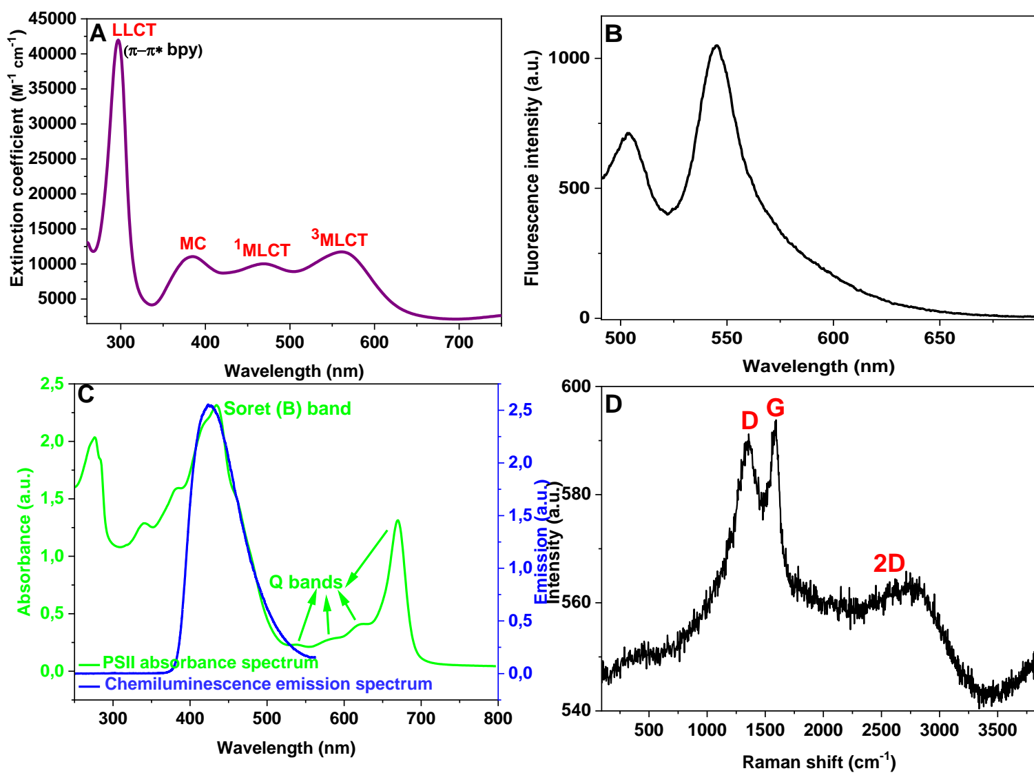
Figure 3. UV-vis absorbance (A) and fluorescence (B) spectrum of Os complex in degassed DMF ( Os(bpy)_2Cl_2 concentration = 1.10^{-5} M); PSII absorption and luminol CL emission spectra (C); Raman spectrum of macroporous carbon (D)
