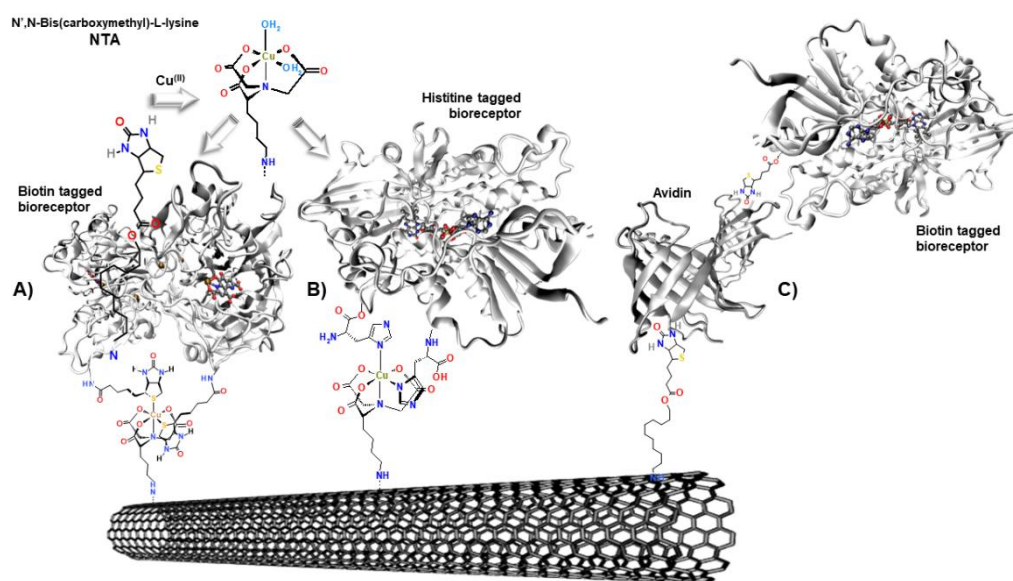
Figure 6: Immobilization of bioreceptor units by coordination of A) biotin or B) histitine tagged bioentities on NTA- Cu^{2+} modified nanocarbon based electrodes. C) Historical immobilization strategy using the biotin-avidin-biotin system.
