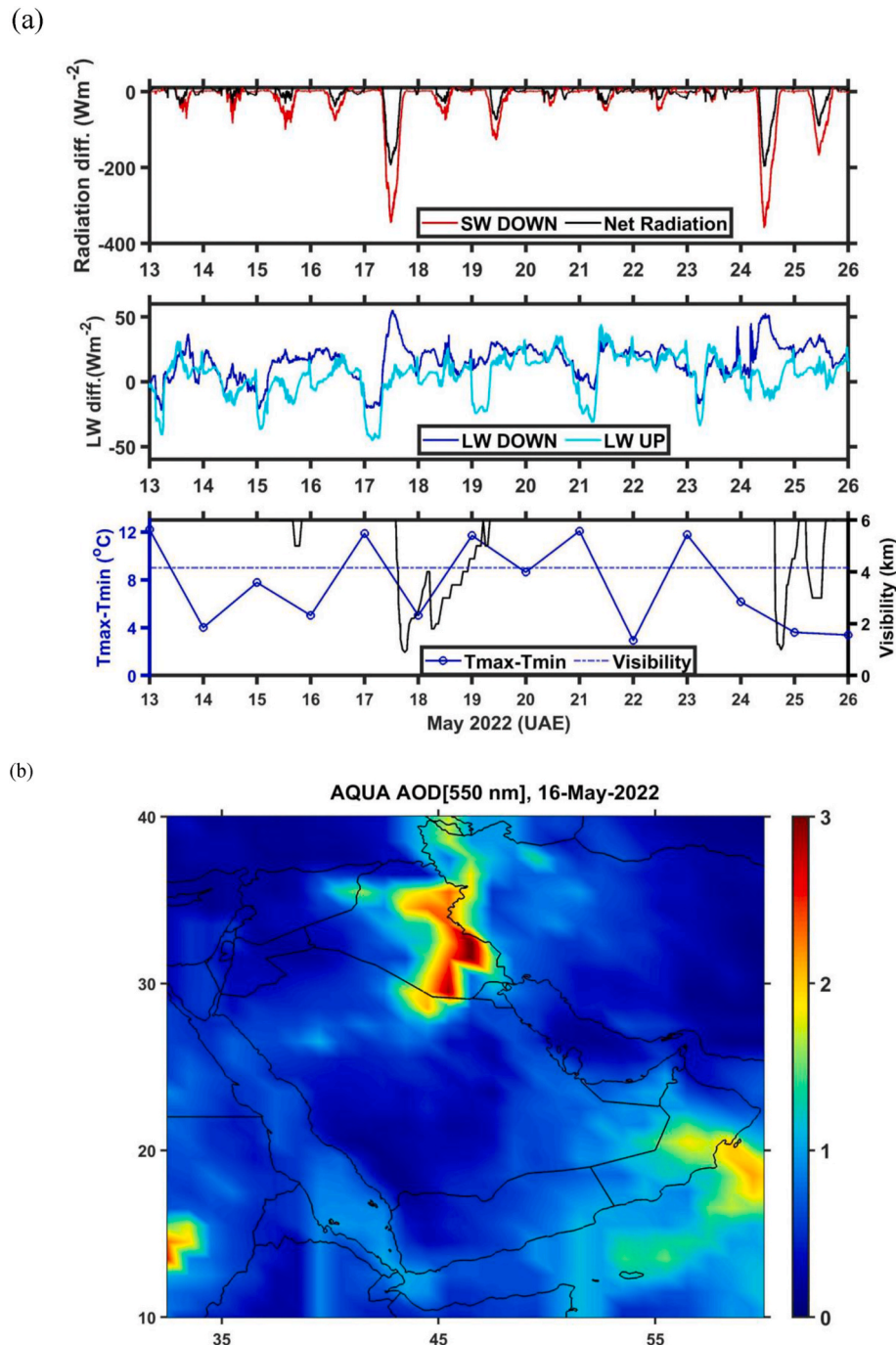
Fig. 7. Radiative impact of dust storms: (a) All-sky surface downwards (red and blue) and upwards (green and cyan) shortwave and longwave radiation fluxes ( \text{W m}^{-2} ) and net radiation flux (black; \text{W m}^{-2} ) as measured by a radiation sensor at Barakah (asterisk in Fig. 1c) from May 13, 2022 at 00 LT to May 26, 2022 at 00 LT. The fluxes plotted are the anomalies with respect to the May 10, 2022 values, a clear/dust-free day. The third panel gives the amplitude of the air temperature diurnal cycle ( ^{\circ}\text{C} ) and horizontal visibility (km) at Barakah (asterisk in Fig. 1c) and Abu Dhabi (cross in Fig. 1c), respectively. The temporal resolution is 1 min for the radiation fluxes and 10 min for the weather fields. (b) AOD at 550 nm from the MODIS instrument on board the Aqua satellite on May 16, 2022. (c) Daily-averaged surface downward shortwave radiation flux (left; \text{W m}^{-2} ) and longwave radiation flux (right; \text{W m}^{-2} ) anomalies on May 16, 2022 from the Clouds and Earth's Radiant Energy System (CERES; Kratz et al., 2014; Kratz et al., 2020) data, available on a 1^{\circ} \times 1^{\circ} grid, with respect to the 2000–2019 May climatology. The white pixels denote missing data. (d) Daily temperature anomalies ( ^{\circ}\text{C} ) at 12 UTC in the bottom 16 km of the atmosphere as measured by radiosondes launched at Abu Dhabi's Airport (cross in Fig. 1c) for May 2022. The anomalies are computed with respect to the 2009–2019 May climatology.
