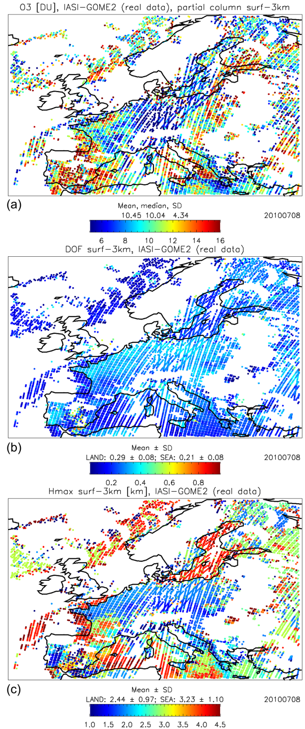
Figure 1. Real IASI+GOME-2 retrievals for 8 July 2010. Maps of ozone column density (O 3 -3km) [DU] (a), the degree of freedom (DOF-3km) (b), and the altitude of maximum sensitivity (Hmax-3km) [km] calculated between the surface and 3 km altitude (c). White areas indicate a lack of measurements due to the presence of relatively high cloud fraction (> 30%), unavailability of satellite data or invalid retrievals.
