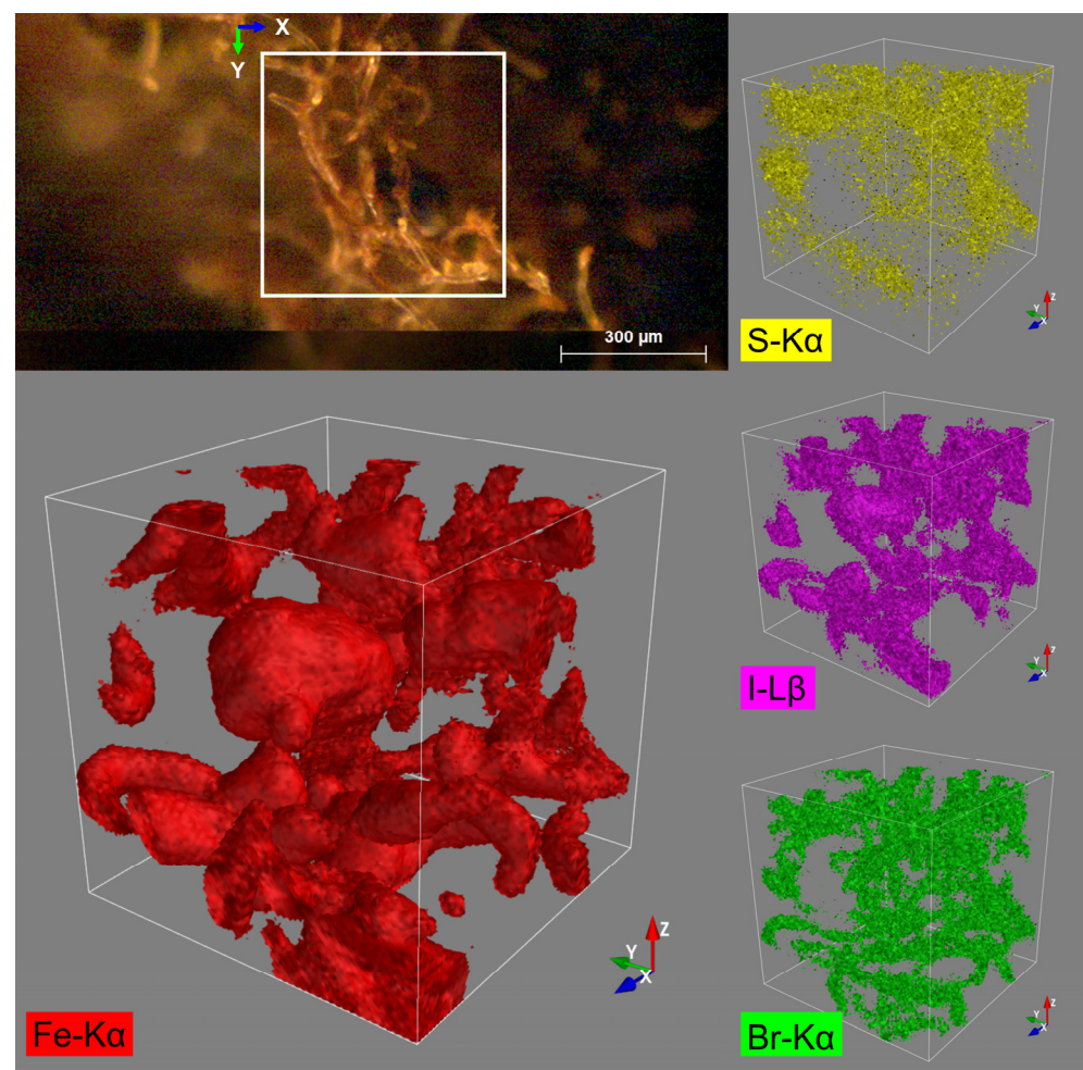
Figure 12. The 3D distribution images of the elements S (K \alpha ), Fe (K \alpha ), Br (K \alpha ), and I (L \beta ) within an analyzed volume of 500 \times 500 \times 500 \mu\text{m} of the FeSpongin sample.
