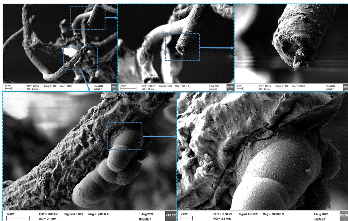
Figure 5. SEM imagery of FeSpongini composite: (A) spongini scaffold, (B,C) crust-like structure covering spongini fiber, (D,E) clearly visible iron mineral conglomerates built on spongini fiber.
