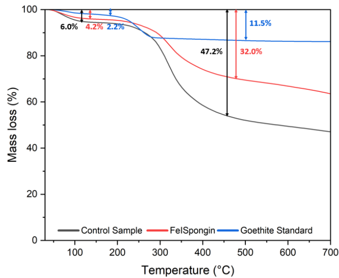
Figure 10. Thermogravimetric (TG) curves of control sample, FeSpongini composite, and goethite standard.
