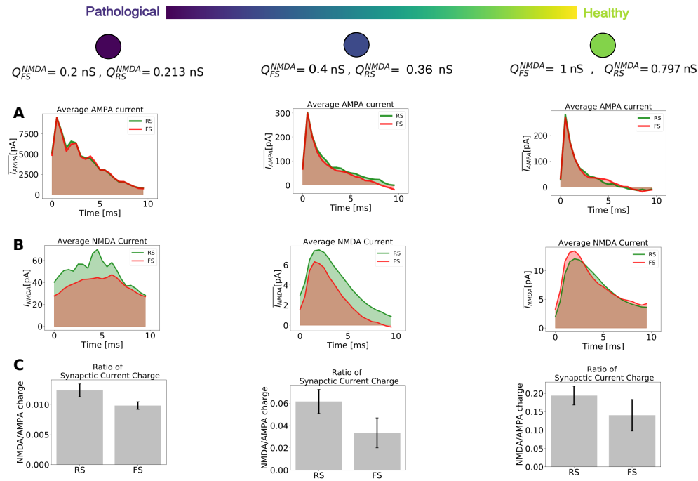
Fig. 4. Excitatory synaptic currents with respect to different levels of NMDA channels block. As in Figure 3, higher values of synaptic strengths are associated with healthy conditions, while lower values of synaptic strengths are associated to pathological conditions supposedly similar to the schizophrenic brain. A) Average AMPA current (for healthy and pathological conditions) of two randomly picked neurons : RS (green) and FS (red). B) Average NMDA current (for healthy and pathological conditions) of two randomly picked neurons : RS (green) and FS (red). C) Ratio of NMDA and AMPA charges for RS and FS cells (for healthy and pathological conditions). The synaptic charge ratio of each neuron was calculated separately. The Bars indicate the mean and the standard deviation among the RS and FS population.
