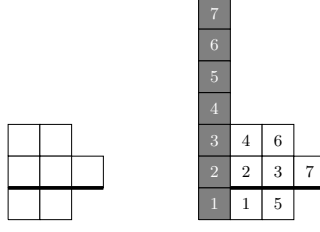
FIGURE 1. (k = 2, \mu = (3, 2, 0, 0, 0, 0)) -diagram and a k -Young tableau of shape (k, \mu)
