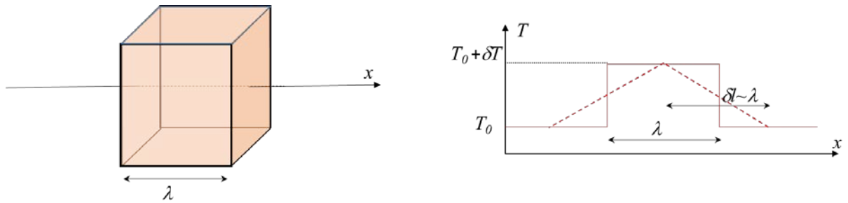
Figure 3. Small volume \delta V of length \lambda corresponding temperature profile (red line) and local approximate temperature gradient (red dotted line)
