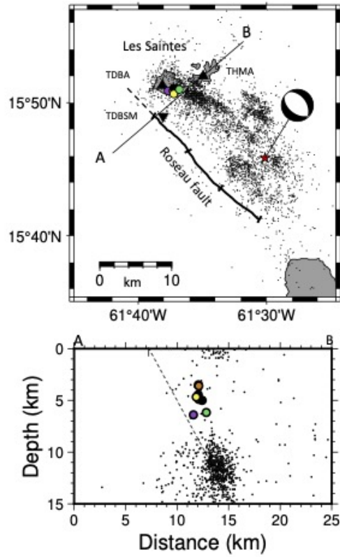
Figure 10. Locations of the multiplets (colored circles) in plan and section in the seismo-tectonic context of the November 11, 2004 earthquake. The locations of the aftershocks are in black (Bazin et al., 2010). The focal mechanism and the location of the mainshock (red star) are from (Feuillet et al., 2011).
