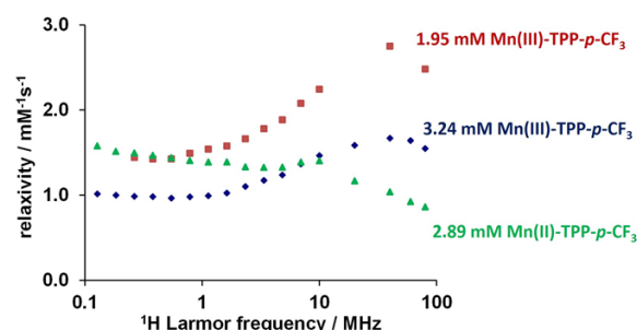
Figure 10. ^1\text{H} NMRD profiles recorded at 298 K in 20% DMSO and 80% water mixture for Mn(III)-TPP- p -CF 3 at 3.24 mM (blue ♦) and 1.95 mM (red ■) concentrations and for Mn(II)-TPP- p -CF 3 at 2.89 mM concentration (green ▲).
