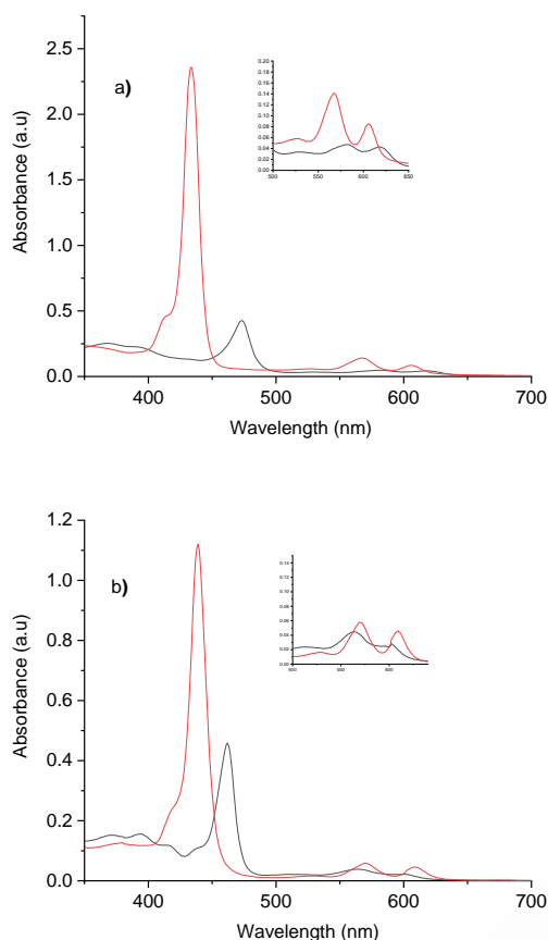
Figure 7. UV-Vis spectra showing the re-oxidation of Mn(II)-TPP- p -CF 3 upon air exposure after 1 h, at 25°C: a) THF and b) DMSO, Mn(II)-TPP- p -CF 3 (red line), Mn(III)-TPP- p -CF 3 obtained after air exposure (black line).
