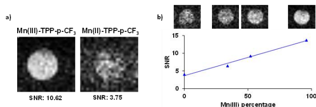
Figure 9. a) ^{19}\text{F} MRI phantom images acquired at 1.1 mM Mn(III)/(II)-TPP- p -CF 3 concentration in DMSO. b) Monitoring reoxidation of Mn(II)-TPP- p -CF 3 ( C_{\text{MnL}} = 1.6 mM) by air oxygen: signal to noise ratio (with respect to the Mn(III)-TPP- p -CF 3 peak) as a function of the oxidized Mn(III)-TPP- p -CF 3 content (%); the signal of the Mn(II) complex was saturated with a selective pulse. B = 7T; TR: 60 ms; TE: 1.3 ms; FA: 90°; NA: 256; acquisition time 8 min 11 s.
