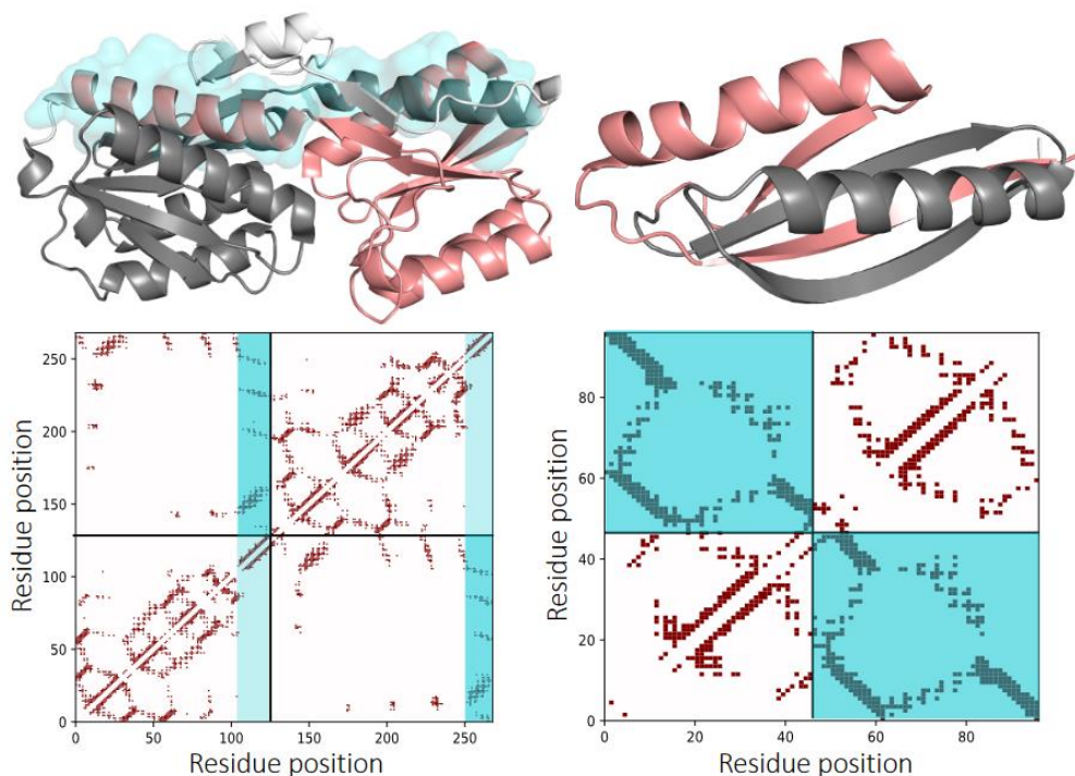
Figure 5. Examples of the structures and their contact maps for swapping identification. Each map is divided into four squares containing intra- and inter-repeat contacts of two repetitive units. Regions with contacts of interest are shown in blue: on the left, these are regions where one repeat has contacts only with another one for the structures with the repeat length over 55 residues (PDB 1abe:A) and, on the right, these are regions where one repeat has numerous contacts with another one for structures with the repeat length less than 55 residues (PDB 1j27:A). The source code of C2_swapping program is available at https://github.com/mlkndt/c2 .
