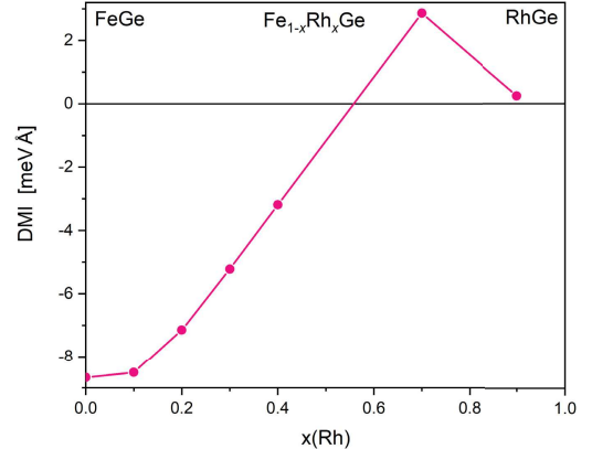
Figure 3: The estimated value of DM interaction in the \text{Fe}_{1-x}\text{Rh}_x\text{Ge} compounds.
