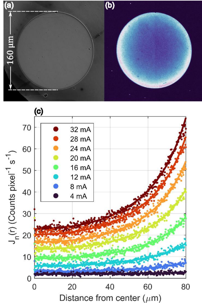
Fig. 3: (a) LEEM image of the circular aperture at zero diode bias prior to cesiation. The electron landing energy is -0.20 eV and the sample is close to in focus. (b) The emitted electron intensity profile at diode current of 32 mA. The emitted electron intensity is clearly larger near the contact metal outer edges and decreases towards the center of the aperture. The contact metal does not emit electrons. (c) The emitted electron intensities at various diode currents plotted (solid circles) fitted to Eq. 9 (solid lines), showing good agreement between data and the analytical solutions by Joyce and Wemple. 1
