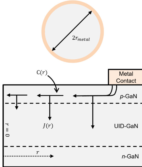
Fig. 1: Schematic of the device solved analytically in Ref. [1], which is of experimental interest in this work. A circular aperture with center at r = 0 is contacted at the edge at radius r_{metal} by an annular metal contact of finite width.
