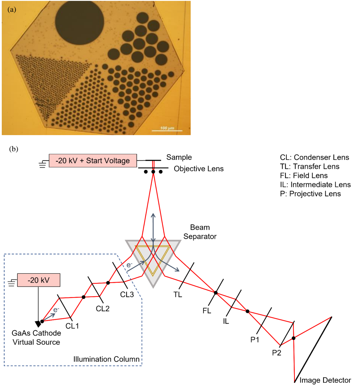
Fig. 2: (a) Optical micrograph of the device fabricated, showing the hexagonal shaped p-contact with multiple circular open apertures of various radii. (b) Schematic of the LEEM tool – with illumination column, sample chamber and imaging column depicted. In EEM mode, the illumination column is not used.
