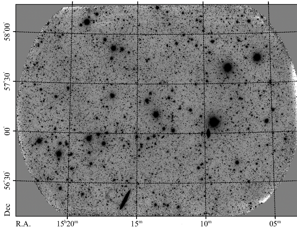
Figure 4. Coadded image of Condor field 6184. Image is smoothed by Gaussian kernel of FWHM = 2.5 pix. Total exposure time is 24.1 h. Galaxy NGC 5907 is toward lower centre of image.
