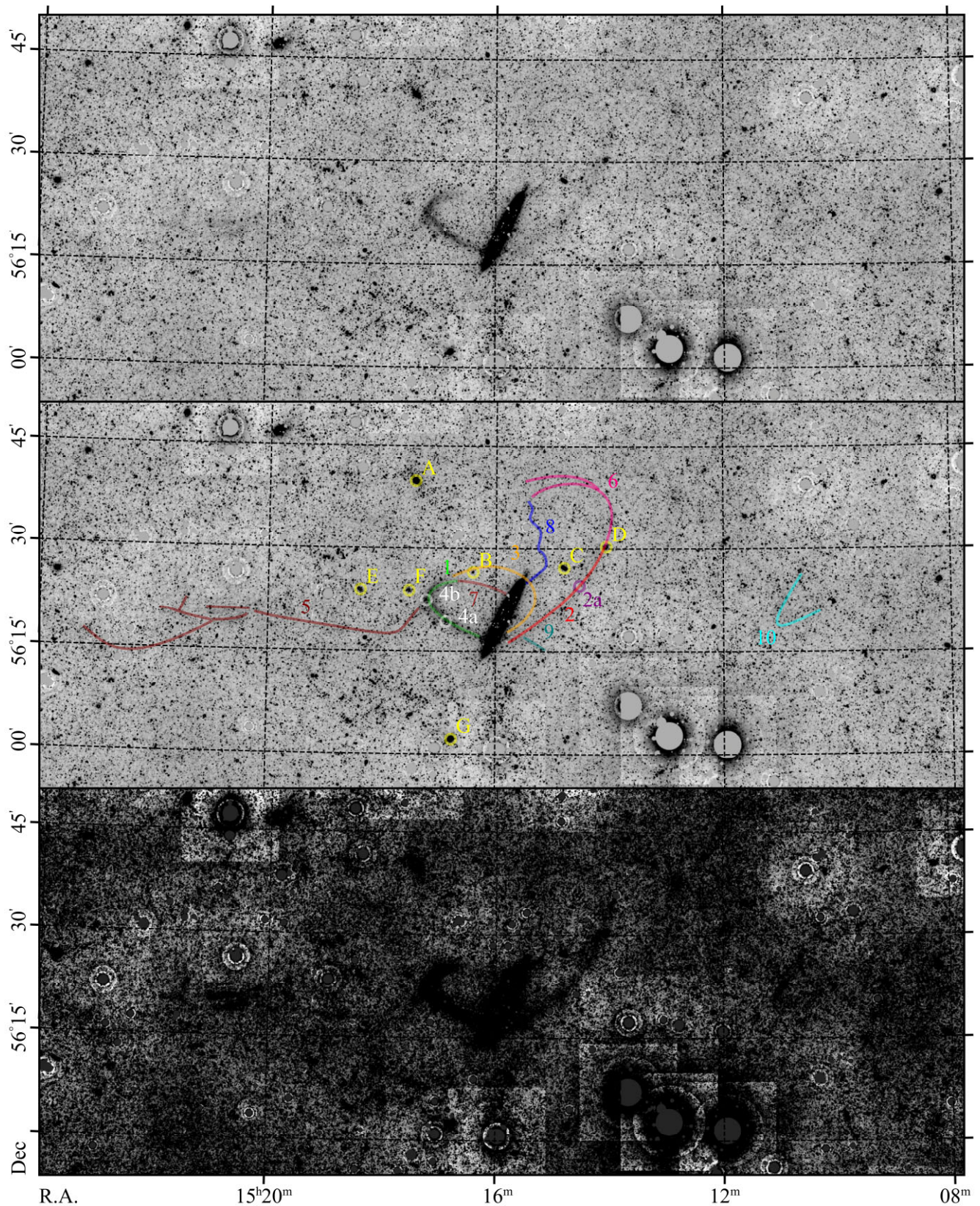
Figure 12. Processed mosaic image of region around NGC 5907 at shallower (top and middle panels) and deeper (bottom panel) stretches. Image is smoothed by Gaussian kernel of \text{FWHM} = 2.5 pix. Middle panel shows schematic representation of features described in Section 6 labelled as follows: 1 (green) eastern stream, 2 (red) western stream, 2a (purple) apparent gap in western stream, 3 (orange) putative second loop of stellar stream, 4a and 4b (white) feature and clump of sources in eastern stream, 5 (maroon) linear feature terminating on patch, 6 (pink) putative extension of western stream, 7 (brown) continuation of eastern stream, 8 (blue) western ‘horn’, 9 (turquoise) southern ‘spur’, 10 (aqua) western ‘hook,’ and A–G (yellow) dwarf galaxies.
