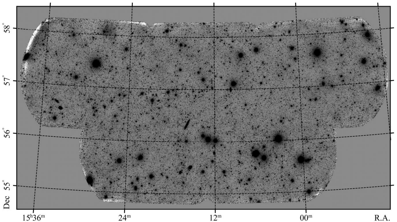
Figure 7. Coadded mosaic of the entirety of the NGC 5866 Group. Image is smoothed by Gaussian kernel of FWHM = 2.5 pix, and angular extent of image is \approx 7.0 \times 3.5 \text{ deg}^2 . Total exposure time summed over all six pointings is 122 h.
