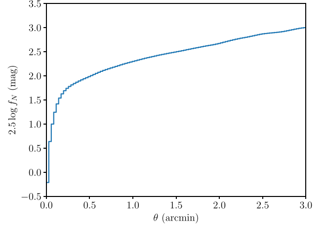
Figure 10. Factor f_N by which standard deviation of background is altered with respect to value obtained considering uncertainty images alone (on a magnitude scale) of the mosaic region versus angular scale \theta .
