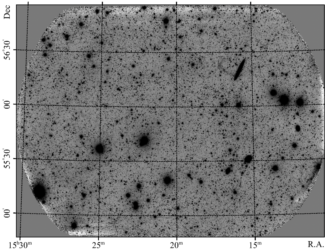
Figure 2. Coadded image of Condor field 6090. Image is smoothed by Gaussian kernel of FWHM = 2.5 pix. Total exposure time is 25.0 h. Galaxy NGC 5907 is toward upper right of image.
