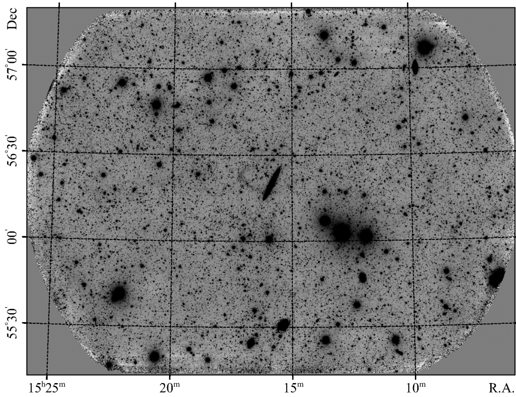
Figure 6. Coadded image of NGC 5907. Image is smoothed by Gaussian kernel of FWHM = 2.5 pix. Total exposure time is 21.4 h. Galaxy NGC 5907 is near centre of image.
