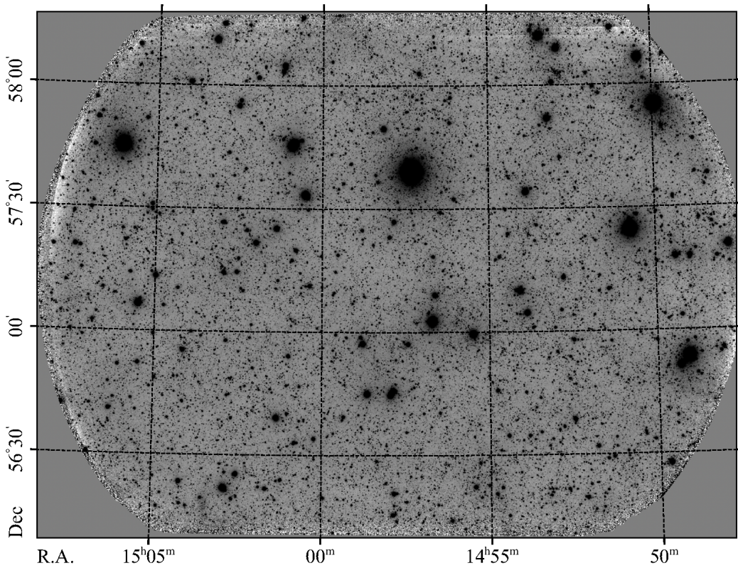
Figure 3. Coadded image of Condor field 6183. Image is smoothed by Gaussian kernel of FWHM = 2.5 pix. Total exposure time array is 19.7 h.
