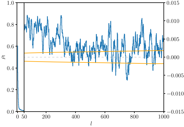
Figure 9. Correlation coefficient \rho_l (blue curves) together with positive and negative one standard deviation uncertainties (orange curves) of mosaic region for pixel lags over intervals l = 0 through 50 (left panel and left scale) and l = 50 – 1000 (right panel and right scale).
