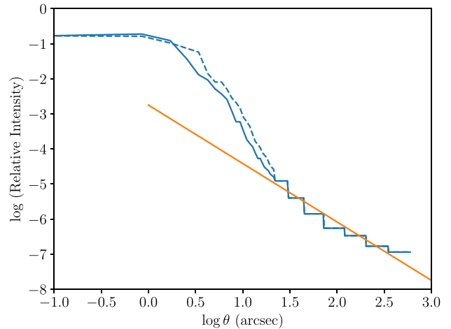
Figure 11. Radial cut of representative example of PSF determined according to description of Section 4, normalized to unit area. Solid and dashed curves show PSF in two opposite directions. Orange line segment show \theta^{-2} radial profile.
