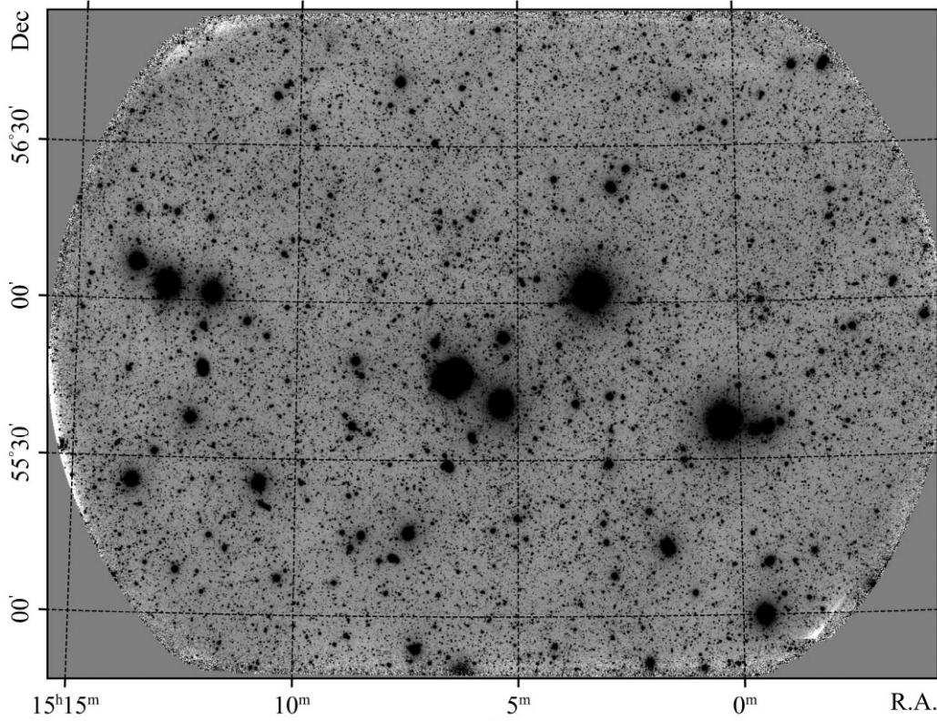
Figure 1. Coadded image of Condor field 6089. Image is smoothed by Gaussian kernel of FWHM = 2.5 pix. Total exposure time is 22.7 h.
