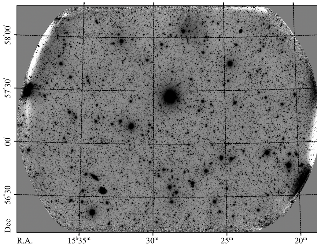
Figure 5. Coadded image of Condor field 6185. Image is smoothed by Gaussian kernel of FWHM = 2.5 pix. Total exposure time is 9.1 h.
