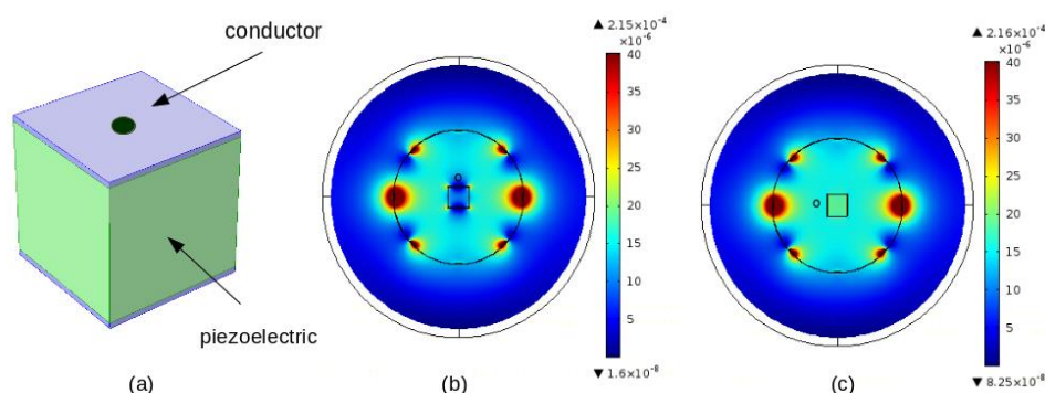
Figure 4. Distribution of the MRI RF magnetic field in the situation of insertion of a piezoelectric coated by electrodes (a) structure configuration, (b) distribution with electrodes perpendicular to the field, and (c) distribution with electrodes parallel to the field [71,72].
