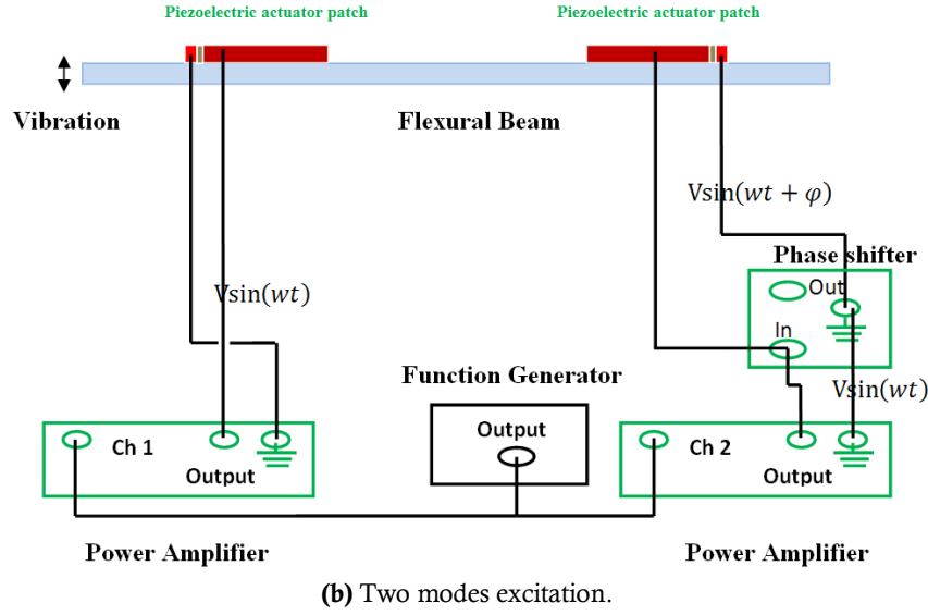
Figure 1. Schematics of one and two mode excitations in the case of PRBR [4] .
