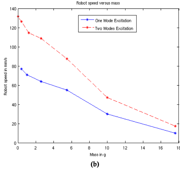
Figure 6. Robot speed versus (a) applied voltage; and (b) embedded mass, one mode and two modes excitation [4] .
