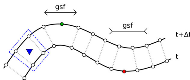
Figure 4. Wave fronts are defined as a string of nodes (circles) and interpolated between to form a smooth wave front (solid line). As the wave front progresses (dashed lines), the distance between neighbouring nodes can increase or decrease. This is the gsf, that is, the node density of the wave front with respect to the initial density. If nodes get too close together (red circle), they are removed in the next wave front; if they are too far apart, a node is added (green circle). When two successive wave fronts, t and t + \Delta t , pass over a receiver (triangle), the arrival time and other properties are calculated by interpolating between the enclosing nodes on each wave front.
