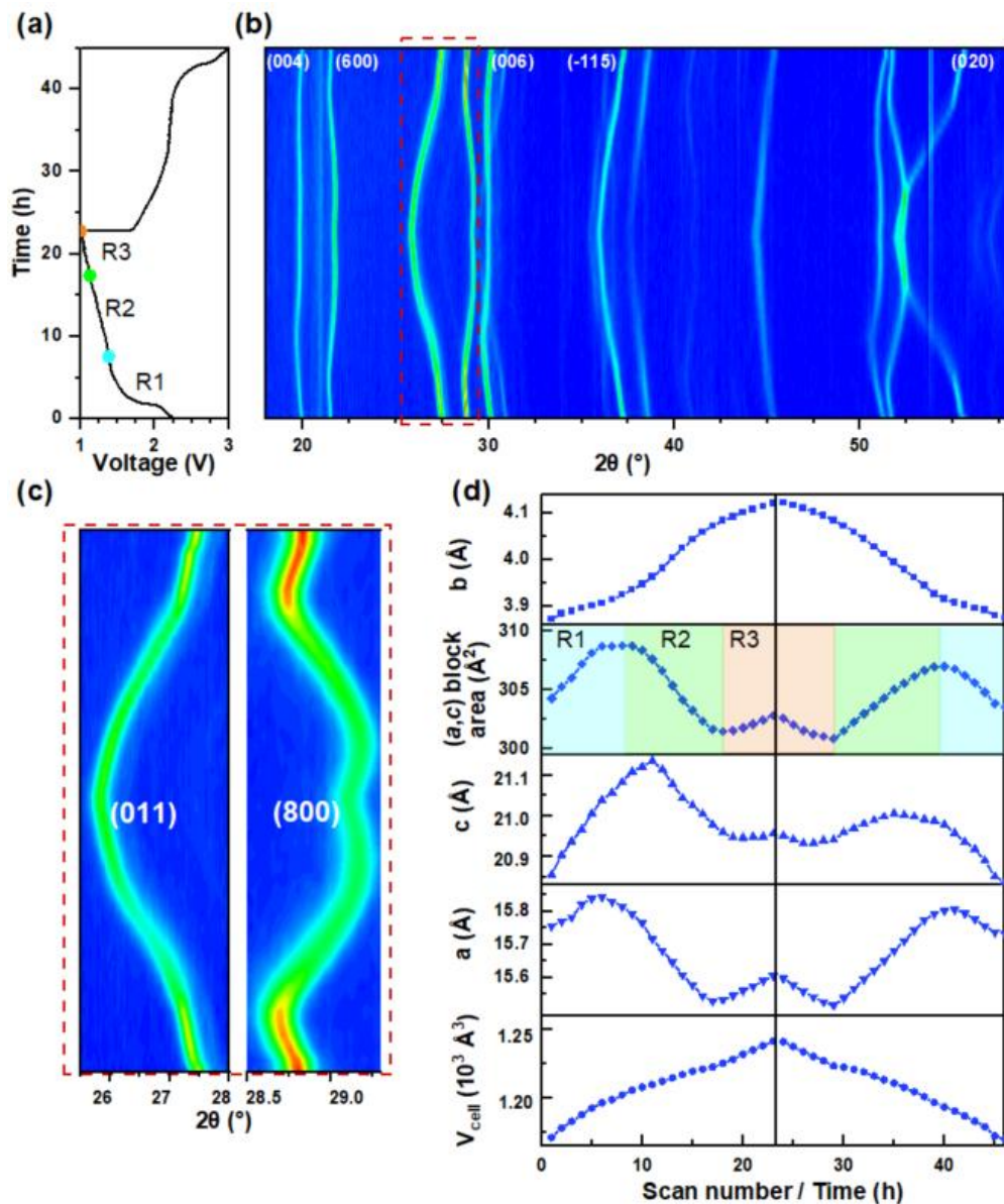
Figure 5. The charge-discharge curve (a) and corresponding 2-dimensional contour plot of operando XRPD patterns for monoclinic \text{FeNb}_{11}\text{O}_{29} (b), magnified view of (800) and (011) reflections (c), and the evolution of lattice parameters, (a,c) block area and unit cell volume during cycling (d).
