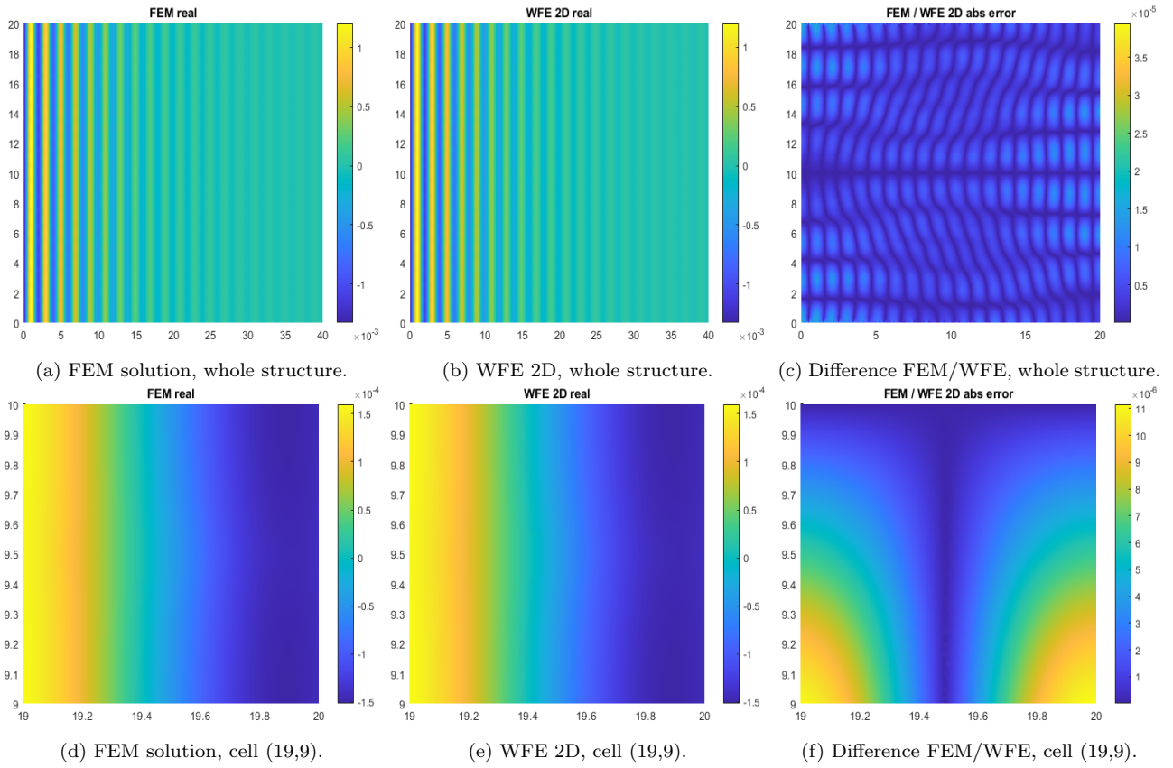
Figure 13: Comparison of the FEM and WFE 2D solutions at 180Hz for a uniform excitation on the left boundary.
