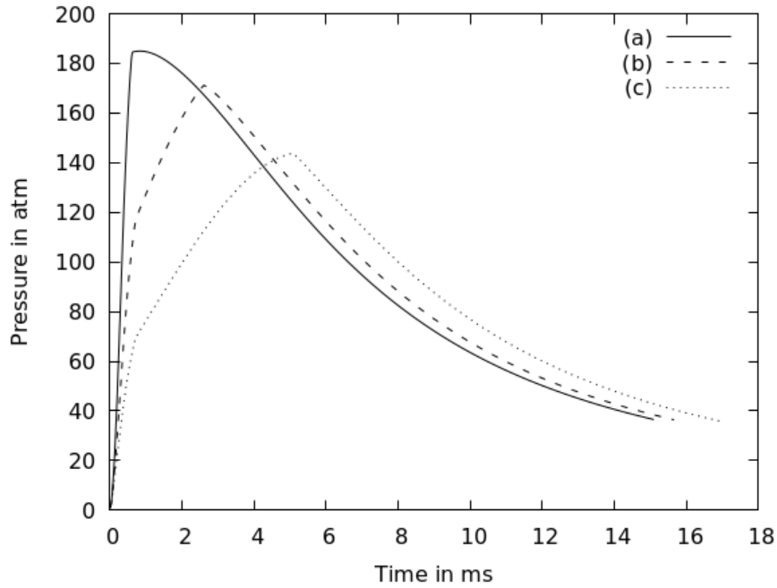
Figure 2: Pressure evolution over time for different web thicknesses, (a) 0, 22mm, (b) 0, 26mm, (c) 0, 3mm.
