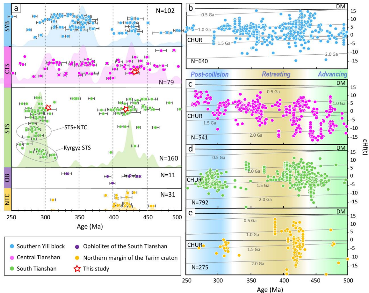
48 49 572 50 573 Fig. 13 (a) Sketch illustration and relative density curves of compiled radiometric ages of 500-250 Ma 51 574 magmatic rocks and ophiolites in southern Yili block (SYB), Central Tianshan (CTS), South Tianshan 52 575 (STS) and northern margin of the Tarim craton (NTC; see data sources in Table S4). (b-e) Compiled zircon 53 576 Hf isotopic compositions from Paleozoic magmatic rocks in SYB, CTS, STS and NTC (see data sources in 54 577 Table S5). 55 56 57 58 59 578
