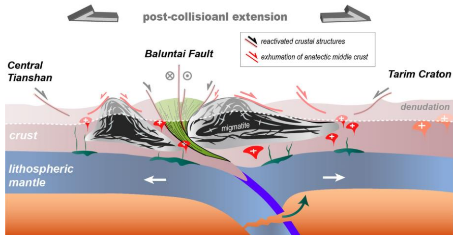
53 943 54 55 944 Fig. 17 Simplified geodynamic model showing the Paleozoic tectonic and magmatic evolution of the 56 Central and South Tianshan (modified from Zhong et al., 2019 ). (a) Silurian-Early Devonian retreating 57 945 subduction of the Paleo-Tianshan Ocean resulted in the opening of the South Tianshan back-arc basin, and 58 946 separation of the Central Tianshan from the Tarim craton, associated with extensional magmatism. (b) From 59 947 60 61 62 63 64 65
