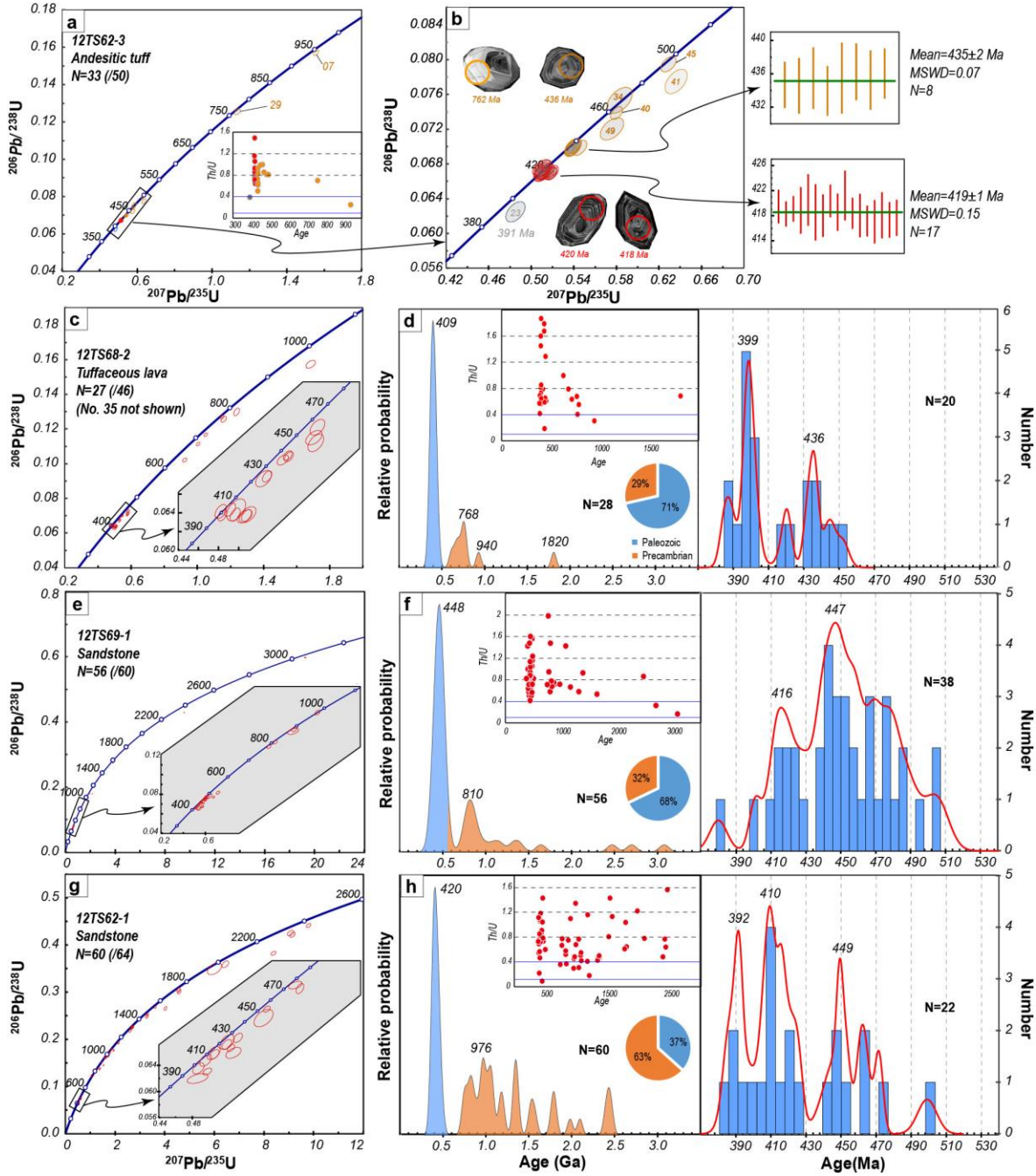
475 476 Fig. 10 Zircon U-Pb Concordia diagrams (a-c, e and g), relative density curves and histograms (d, f and h), 477 and Th/U ratios vs. U-Pb age plots (insets of d, f and h) for volcaniclastic rocks of the Chahan-Wusu 478 section. The CL images of all dated zircons is shown in supplementary Fig. S5.
