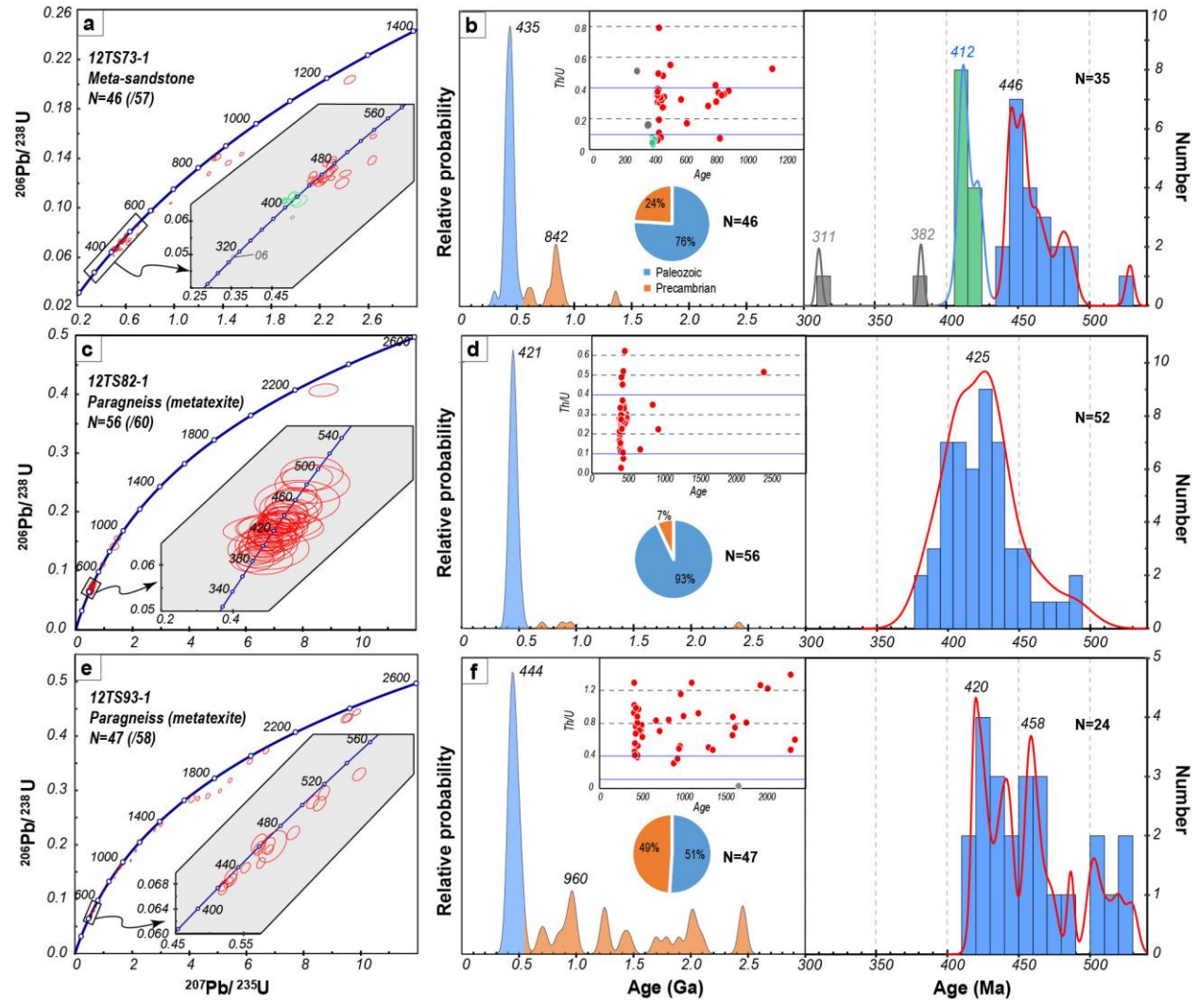
445 Fig. 9 Zircon U-Pb Concordia diagrams (a, c and e), relative density curves and histograms (b, d and f), 446 and Th/U ratios vs. U-Pb age plots (insets of b, d and f) for clastic rocks of the Kerguty section. The CL 447 images of all dated zircons are shown in supplementary Fig. S4. 448
