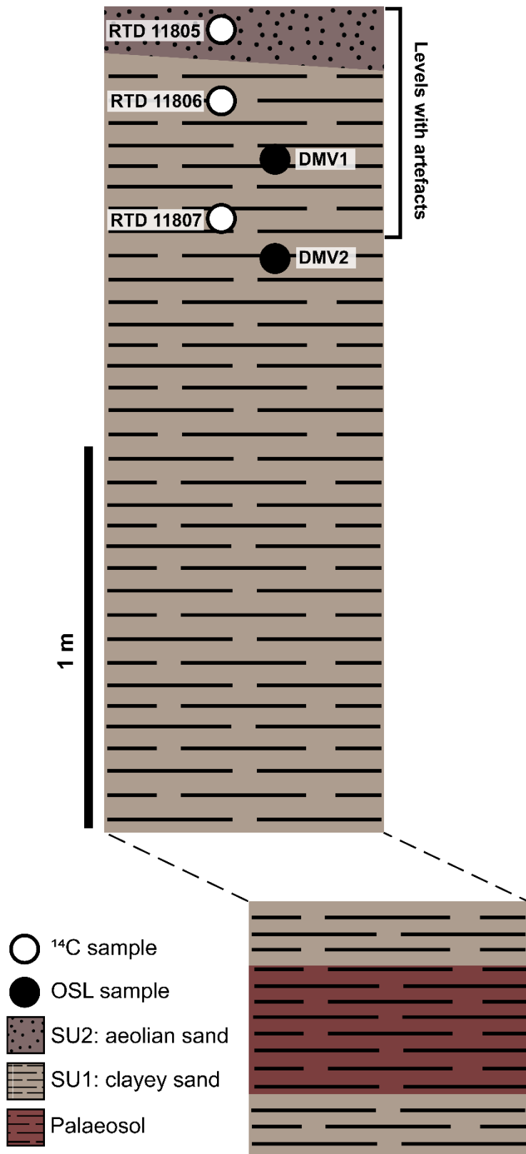
FIG. 5. Damvlei stratigraphic sequence exposed in the donga profile, showing the location of radiocarbon ( 14 C) and OSL dating samples. All dating samples were collected in the excavation trench of Units 1-4 except for DMV1, which was collected from the stratigraphic profile. The red palaeosol, visible at other locales in the donga, was not reached in the stratigraphic profile.
