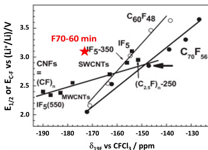
Figure 11. Reduction potential at mid-discharge as a function of the 19 F chemical shift of the C-F bonds of several materials taken from [40]. The cells used 1M LiClO 4 in PC electrolyte. The compound F70-60 min is represented by the red star. IF 5 means room temperature graphite prepared with IF 5 catalyst and its post-treatment temperature is added, e.g., IF 5 -350 was post-fluorinated with pure F 2 gas at 350 °C. The same notation is used for graphite fluoride with (C 2.5 F) n structural type.
