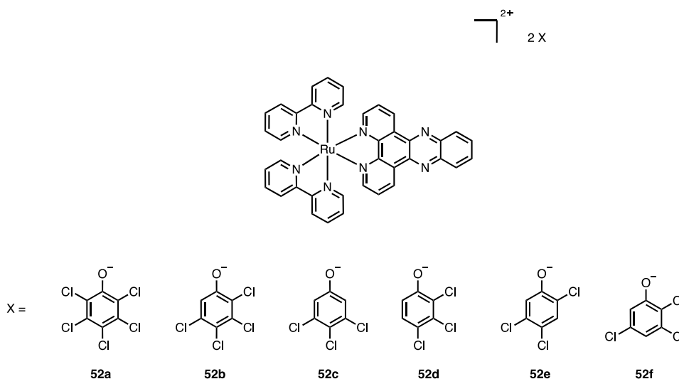
Figure 19. Using lipophilic ion-pairs allows for an increased cellular uptake and nucleus accumulation of [\text{Ru}(\text{bpy})_2(\text{dppz})]^{2+} .
