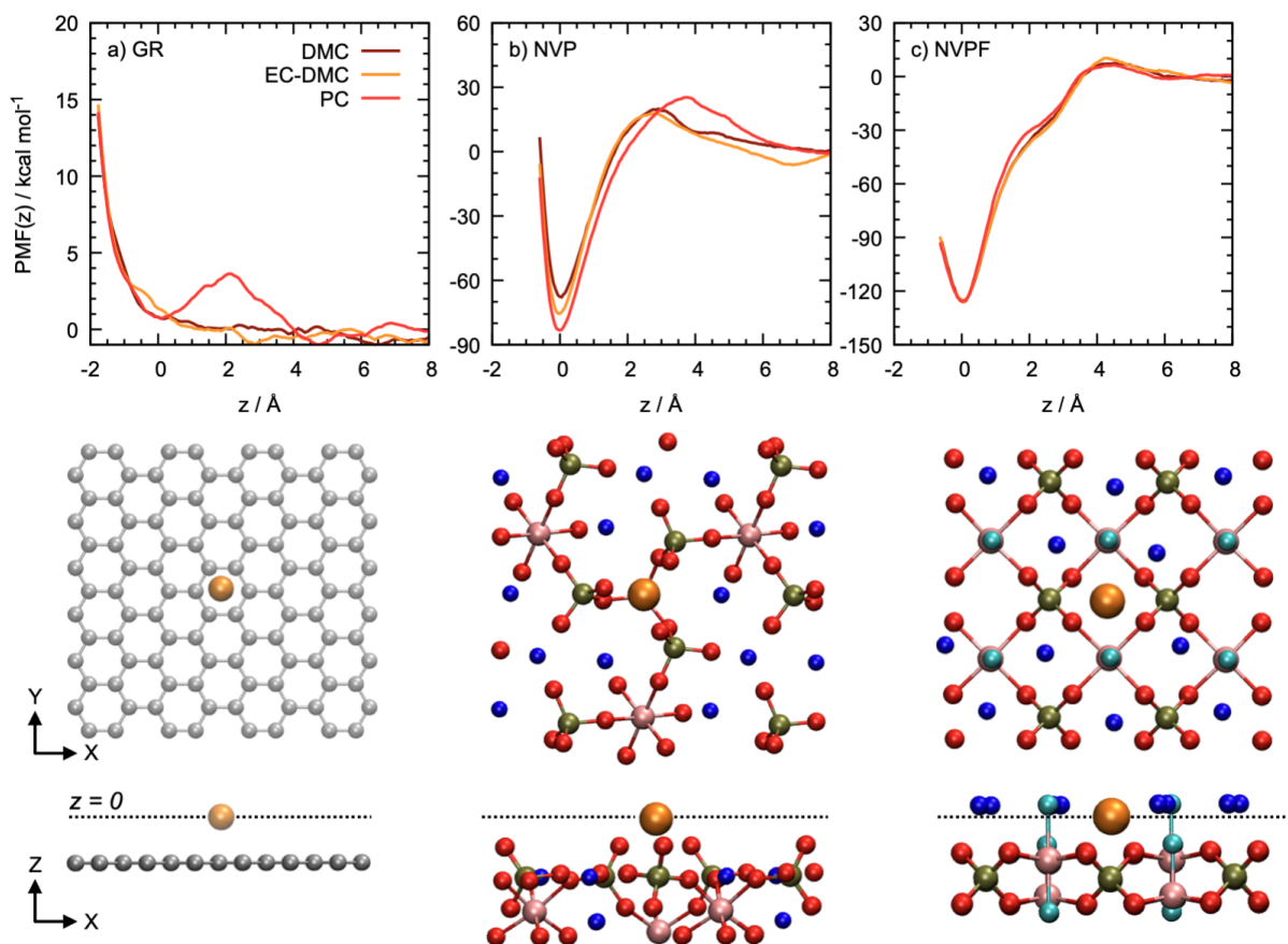
Figure 6: Potential of mean force of approaching a single Na + ion to the graphite (a), NVP (b), and NVPF (c) electrode in different solvents. As a reference ( z = 0 ), the minimum of each PMF is considered, corresponding to the most energetically favorable position of the Na + ion, as illustrated by the simulation snapshots.
