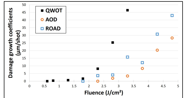
Fig. 6. Evolution of numerical damage growth coefficients in s -polarization as a function of the fluence following the three mirror designs.
