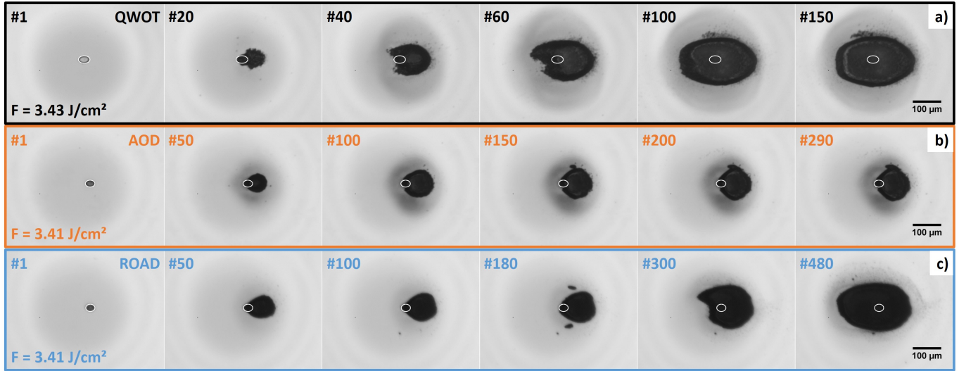
Fig. 3. Microscope acquisitions of the evolution of the damaged area. Damage growth experiments were performed on (a) QWOT design, (b) AOD, and (c) ROAD at a fluence of approximative 3.41 J/cm 2 in s -polarization. See Visualization 1 for complete sequences.
