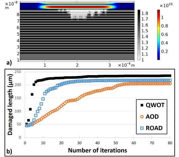
Fig. 5. (a) Example of a numerical damage growth sequence on the AOD after 15 iterations with an incident fluence of 3.8 \text{ J/cm}^2 in s -polarization. The color scale represents the intensity of the incident beam, the gray scale represents the refractive index. (b) Evolution of length of the damage site through the entire sequence for the three mirror designs at a fluence of 3.3 \text{ J/cm}^2 . Only the first 80 of the 200 iterations are displayed.
