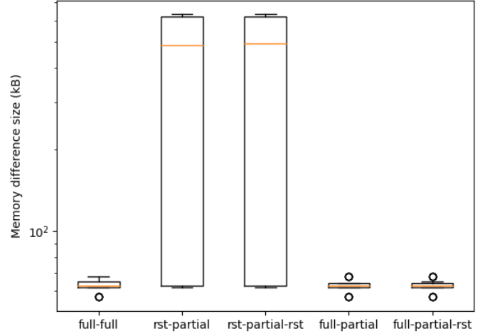
Figure 10: Illustration of memory difference size for each memory snapshot strategy for curl with 1 TLS session. Strategies can be divided into two groups: strategies with a full dump allow intra-page granularity, while strategies without a full dump are limited to page-by-page differences.
