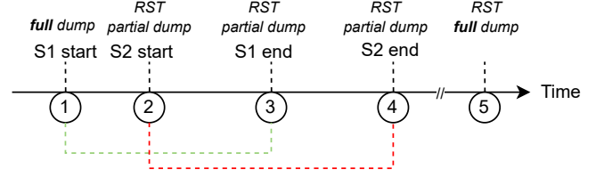
Figure 3: Illustration of changes reconstruction algorithm with the full-partial-rst method. Memory snapshots difference for session 1 (S1) is represented using a green dotted line. Memory snapshots difference for session 2 (S2) is represented using a red dotted line.
