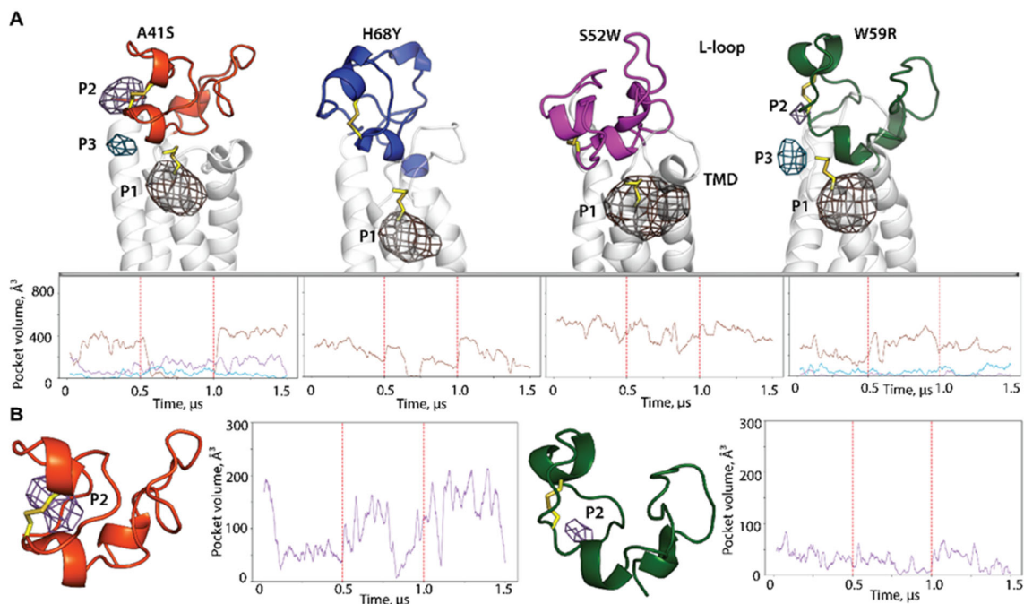
Figure 8. Pockets in hVKORC1 mutants. (A) Pockets localised in four mutants (top) and variation in their volume along the MD simulation (bottom). (B) Pocket P2 localised in L-loop and variation in its volume. (A,B) Protein is shown as a cartoon with the L-loop distinguished by colour: hVKORC1 A41S in orange-red, hVKORC1 H68Y in dark blue, hVKORC1 S52W in fuchsia, and hVKORC1 W59R in dark green. Disulfate bonds and crucial residues are in sticks; pockets are delimited by meshed contours.
