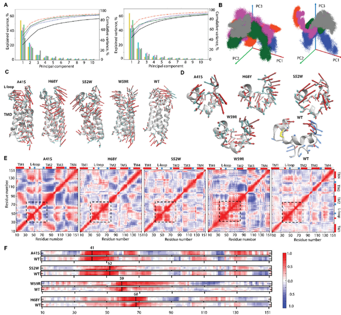
Figure 5. Inherent motion of hVKORC1 and its L-loop. (A) The PCA modes of hVKORC1, describing the TMD and L-loop (left), and only the L-loop (right) global motions, were calculated for the concatenated MD trajectory after least-square fit of the MD conformations to the initial conformation ( t=0 \mu\text{s} ) of the respective domain. Only the \text{C}\alpha -atoms were considered. The bar plot gives the individual explained variance (eigenvalue spectra) in descending order for the first 10 modes. Curves provide the cumulative explained variance. (B) Projection of MD conformations (the TMD and L-loop on the left and the L-loop on the right) in phase space along the first three principal eigenvectors. (A,B) Proteins are distinguished by colour: hVKORC1 A41S in orange-red, hVKORC1 H68Y in dark blue, hVKORC1 S52W in fuchsia, hVKORC1 W59R in dark green, and hVKORC1 WT in grey. (C,D) Atomic components in the first two PCA modes of the analysed hVKORC1 domains are drawn as red (1st mode) and cyan (2nd mode) arrows projected onto the respective average structure shown in a grey cartoon. Only movements with an amplitude \geq 2\text{\AA} are displayed. (E) The inter-residue cross-correlation map calculated for \text{C}\alpha atom pairs after fitting to the respective initial conformation ( t = 0 \mu\text{s} ) of each hVKORC1 using the concatenated trajectories. The L-loop region is delineated by a dashed square. (F) Correlation of each mutated (top) and native (bottom) residue with other hVKORC1 residues. (E,F) Correlated (positive, 1) and anti-correlated (negative, -1) motions between pairs of \text{C}\alpha atoms are represented by a red-blue gradient.
